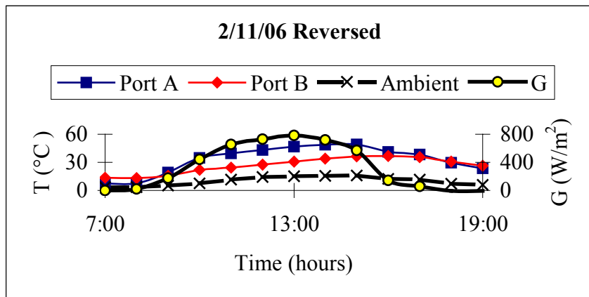
Fig.5 Reversed flow direction
