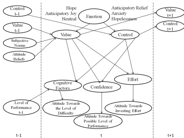
FIGURE 1 OUTCOME-PROSPECTIVE EMOTIONS DBN
