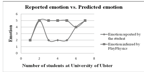
FIGURE 2 RESULTS OF THE PRELIMINARY EVALUATION OF THE OUTCOME-PROSPECTIVE DBN
