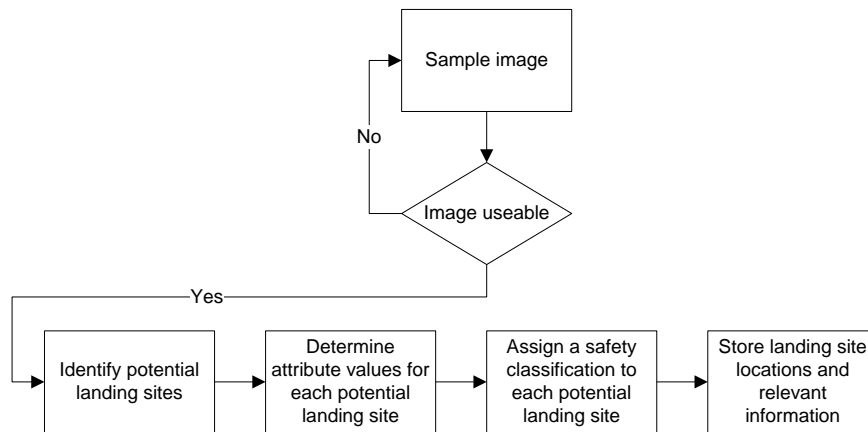
Fig. 2. Safe landing site detection overview
