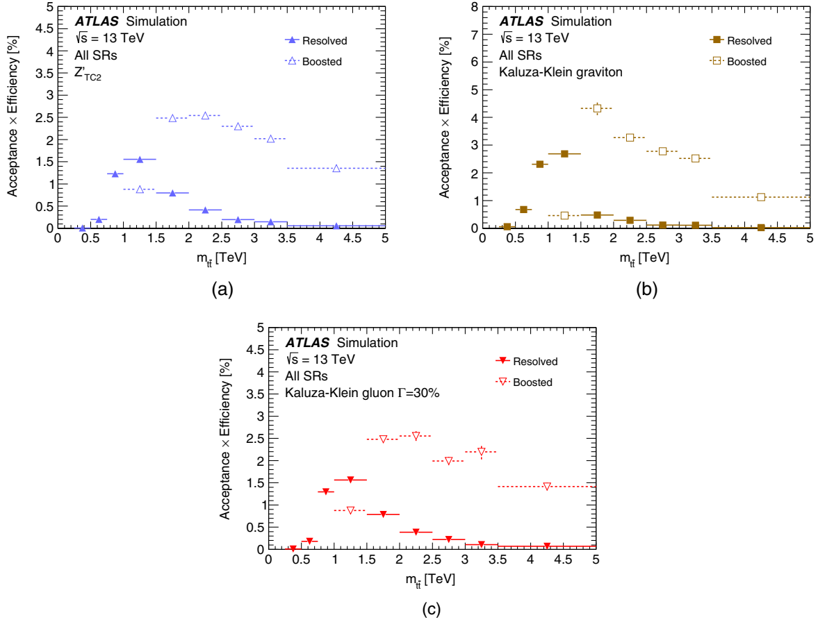
FIG. 5. Acceptance times selection efficiency as a function of m_{\bar{t}t} for all regions A–D in the resolved analysis and the combination of all SRs in the boosted analysis. The momenta of top and antitop quarks evaluated at the generator level before final state radiation are used to define m_{\bar{t}t} . The efficiency calculation includes the branching fractions of the \bar{t}t system into all possible final states. (a) is Z'_{TC2} , (b) is G_{KK} , and (c) is g_{KK} .
