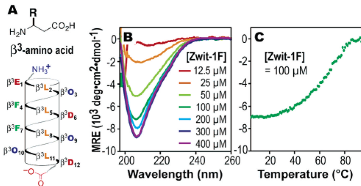
Figure 1. (A) Helical net cartoon of Zwit-1F with \beta -amino acids represented by single-letter codes. \beta^3\text{O} signifies \beta^3 -homomethionine. Concentration (B) and temperature (C) dependent CD spectra of Zwit-1F at 25 ^\circ\text{C} in phosphate buffer (pH 7.1).
