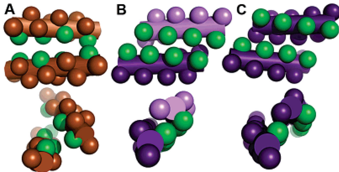
Figure 3. Comparison of leucine packing in (A) the leucine zipper GCN4 20 with the (B) antiparallel and (C) parallel interfaces of Zwit-1F. Helices are represented as solid cylinders, side chains as knobs, and interface leucines colored green.
