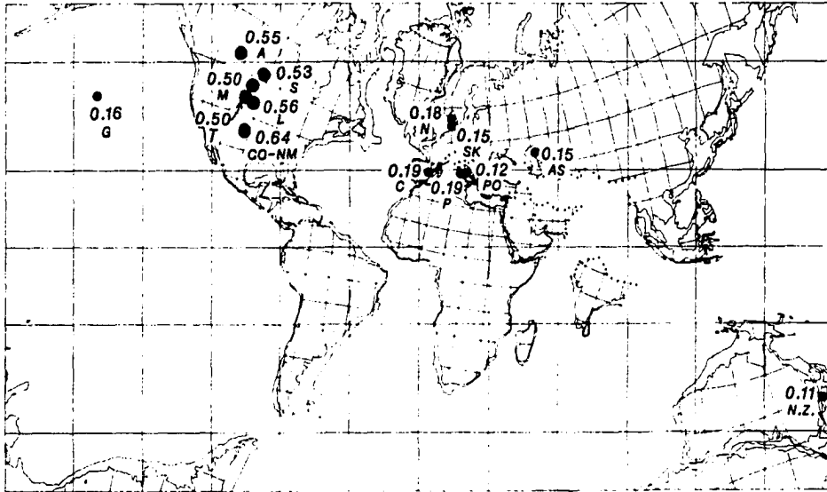
Figure 32.--Paleogeographic map showing the maximum size of shock-metamorphosed quartz grains in K-T boundary rocks. Grain size given in millimeters. Size of locality dots indicates graphically that shock-metamorphosed minerals are several orders of magnitude more abundant at North American boundary sites than elsewhere in the world. Information relative to sites follows: A, Alberta, Canada (Lerbekmo and St. Louis, 1985); S, Saskatchewan, Canada (Nichols and others, 1986); AS, Turkmenia (Badjukov and others, 1986); CO-NM, Raton Basin, Colo., and N. Mex. (fig. 2, this paper); L, Dogie Creek area, Wyo. (Bohor and others, 1987b); T, Teapot Dome, Wyo. (Wolfe and Izett, 1987). Other sites shown by Bohor and Izett (1986) and Izett (1987a) are: M, Brownie Butte, Montana; C, Caravaca, Spain; GPC-3, Giant piston core, North Pacific Ocean; N, Nye Kløv, Denmark; SK, Stevns Klint, Denmark; N.Z., Woodside Creek, New Zealand; P, Pontedazzo, Italy; PO, Petriccio, Italy. Base map (early Paleocene time) from Smith and Briden (1977).
