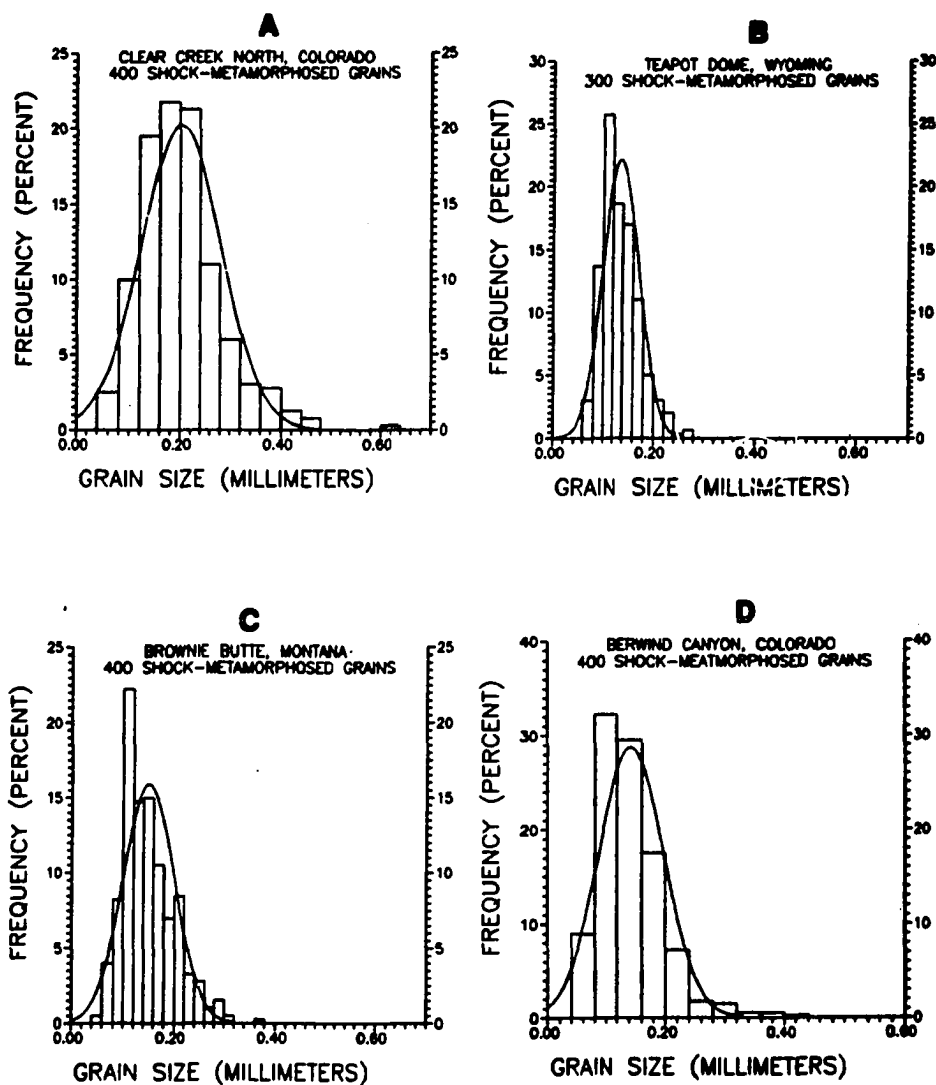
Figure 31.--Frequency diagrams showing size of clastic mineral grains in the K-T boundary impact layer. Superposed chi-square distribution curves are also shown. A, 400 shock-metamorphosed grains from the Clear Creek North, Colo., locality. B, 300 shock-metamorphosed grains from the Teapot Dome, Wyo., locality of Wolfe and Izett (1987). C, 400 shock-metamorphosed grains from the Brownie Butte, Mont., locality. D, 400 shock-metamorphosed grains from the Berwind Canyon, Colo., locality.
