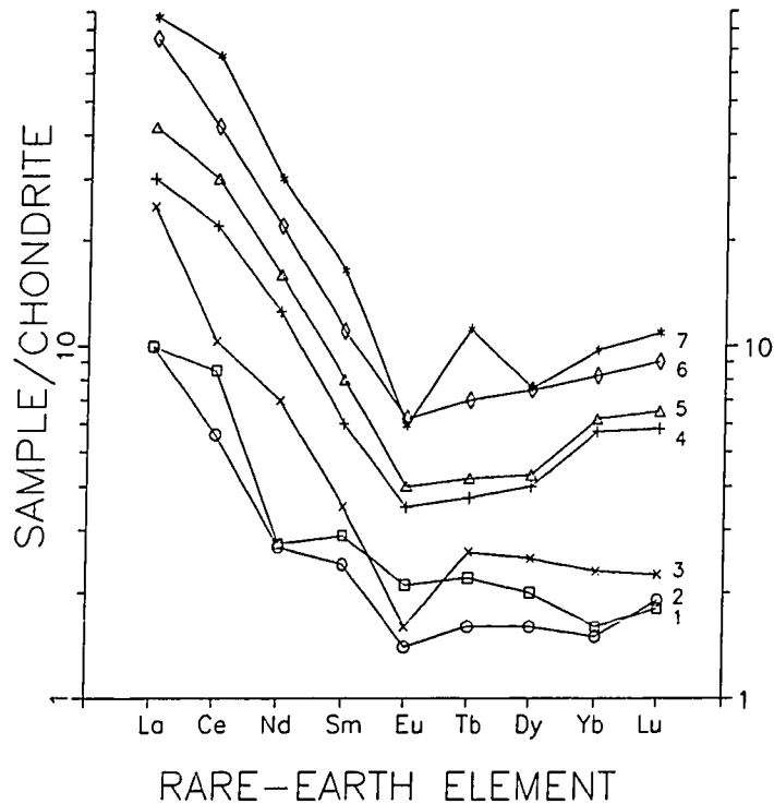
Figure 7.--Rare-earth-element diagram of K-T boundary interval rocks from North America and Europe. A typical kaolinite pattern from Georgia is also shown. Element concentrations normalized to amounts in chondritic meteorites plotted against REE atomic number. 1, Boundary claystone from the Starkville South, Colo.; 2, Boundary claystone at Brownie Butte, Mont.; 3, Boundary claystone residue from Stevns Klint, Denmark (Kastner and others, 1984); 4, Insoluble residue of Tertiary clay directly overlying K-T boundary at Stevns Klint, Denmark (Kastner and others, 1984); 5, Insoluble residue of Cretaceous clay directly underlying K-T boundary at Stevns Klint, Denmark (Kastner and others, 1984); 6, Insoluble residue from K-T boundary claystone at Gubbio, Italy (Kastner and others, 1984); 7, Macon, Georgia, kaolinite of Cullers and others (1975).
