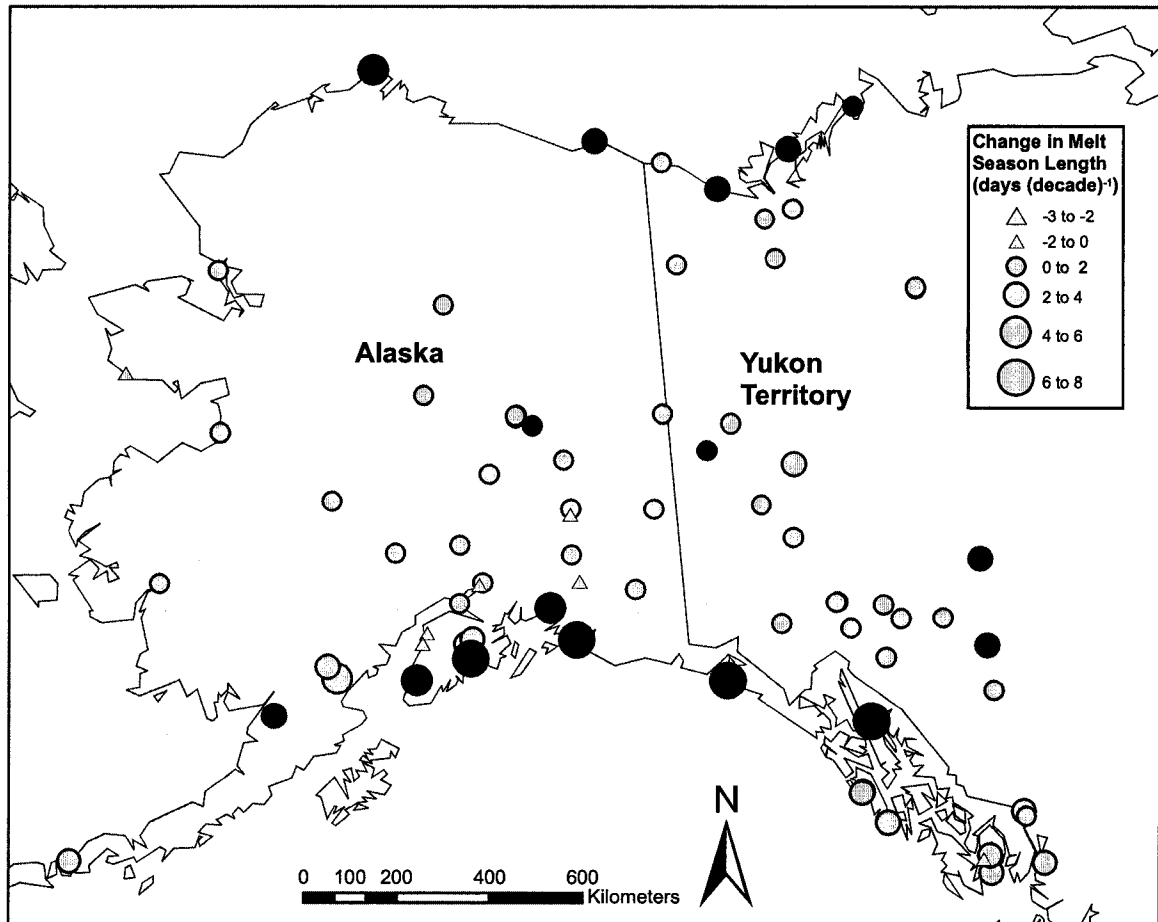
Figure 4.9: Change in melt season length (day (decade) -1 ) in Alaska between 1950 and 2002 at 60 NOAA and 18 Environment Canada climate stations. Black symbols represent changes significant at p < 0.05 .
