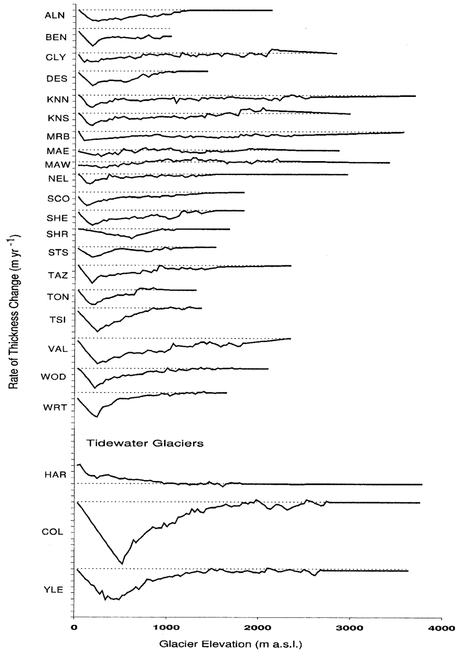
Figure 3.3: Time average rate of glacier thickness change \Delta\dot{h} ( \text{m yr}^{-1} ) as a function of elevation on the glacier at the time of mapping, determined from total thickness changes between 1950/57 to 2001/04. Dotted line represents 0 change and values below this line indicate a reduction in surface elevation relative to the map. Each tick mark on the vertical scale is 1 \text{ m yr}^{-1} of thickness change. Three letter glacier codes are listed in Table 3.2.
