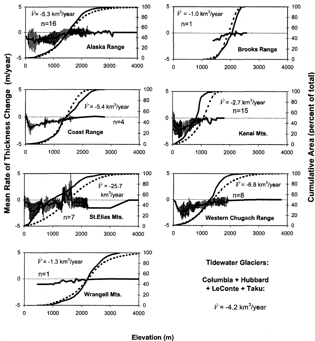
Figure 2.3: Rate of glacier-wide, area-weighted average thickness change versus elevation for the early measurement period (solid black line, left axis), with gray bars indicating measured variations of one standard deviation about the mean. The gray line (right axis) shows regional average curves of cumulative area distribution (%); the dotted black line (right axis) shows cumulative area distribution (%) of glaciers sampled in this study. Comparison of the gray and dotted black lines shows how well we sampled glacier area with elevation for each region. \dot{V} is the total volume change rate for the region, and n is the number of glaciers sampled in the region. Four tidewater glaciers (Columbia, Hubbard, LeConte, and Taku) are treated as separate regions. Similar curves were developed for the recent period.
