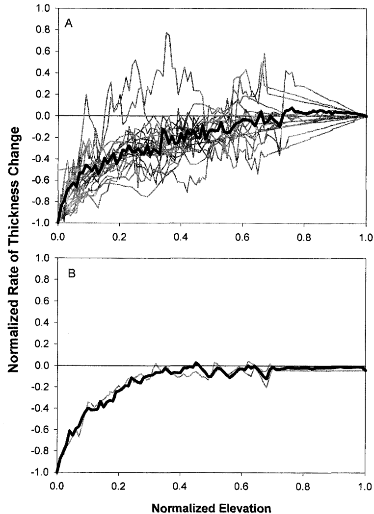
Figure 3.5: Normalized rate of thickness change ( \Delta\dot{h}/-\Delta h_t ) versus normalized elevation ((z-z_t)/(z_h-z_t)) for glaciers of the Western Chugach Mountains, Alaska. Group A is comprised of all glaciers except tidewater glaciers and an obvious outlier, BEN. Group B is comprised of two retreating tidewater glaciers COL and YLE. Gray curves show normalized thickness changes of all glaciers and black curves are area-weighted averages of the gray curves.
