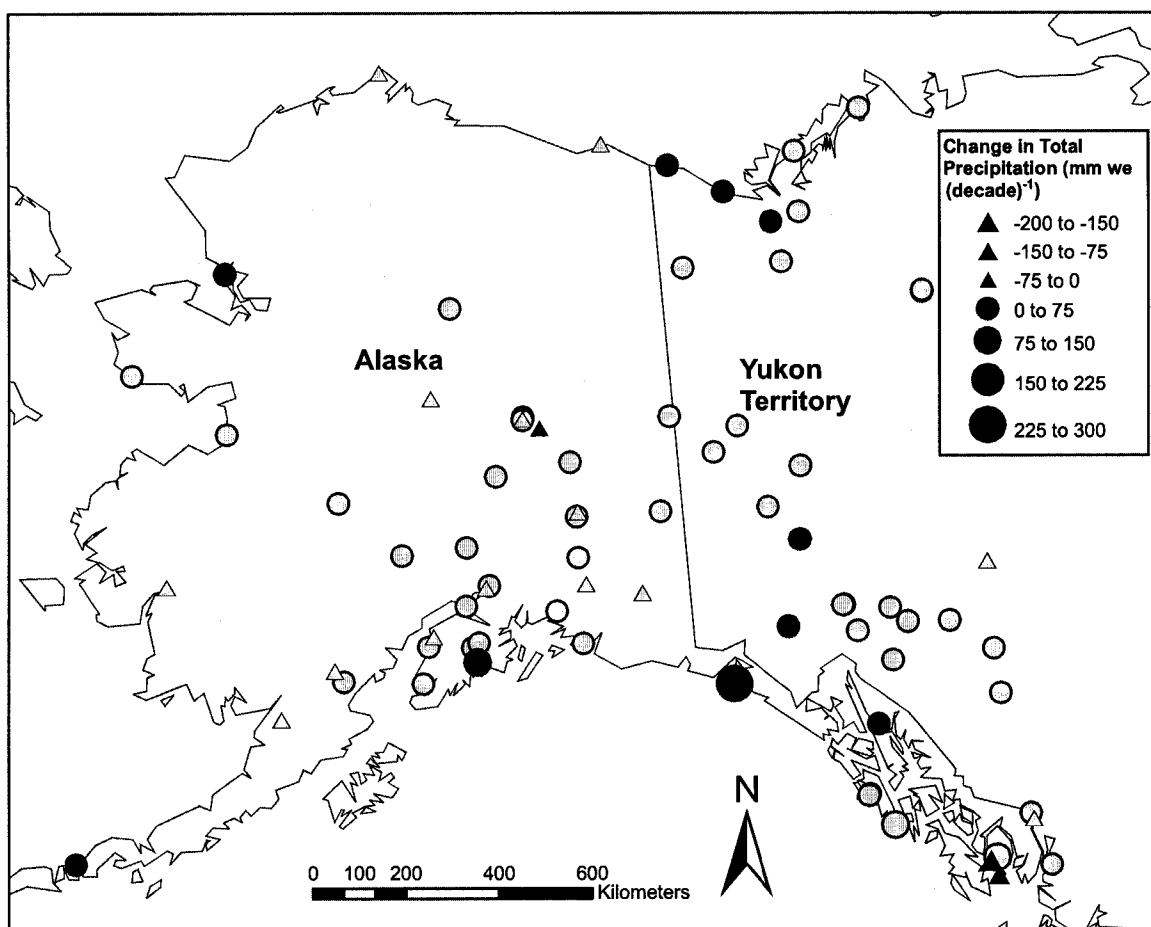
Figure 4.8: Changes in annual total precipitation, 1950 to 2002. Black symbols represent changes significant at p < 0.05 .
