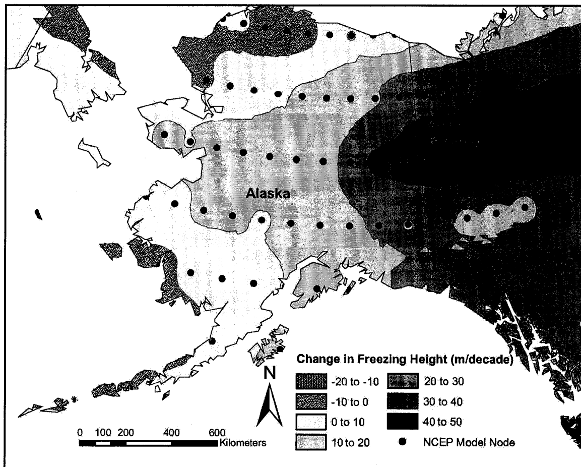
Figure 4.12: Change in winter (October to April) freezing level height ( \text{m (decade)}^{-1} ) in Alaska between 1950 and 2002.
