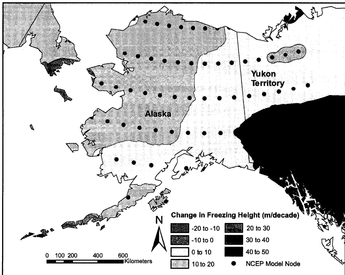
Figure 4.11: Change in summer (May to September) freezing level height ( \text{m} (\text{decade})^{-1} ) in Alaska between 1950 and 2002.
