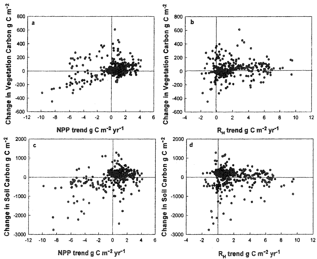
Figure 3.6: Relationship between selected pools and fluxes: a) changes in vegetation carbon vs. change in NPP, b) changes in vegetation carbon vs. change in RH, c) changes in soil carbon vs. change in NPP, d) changes in soil carbon vs. change in RH.
