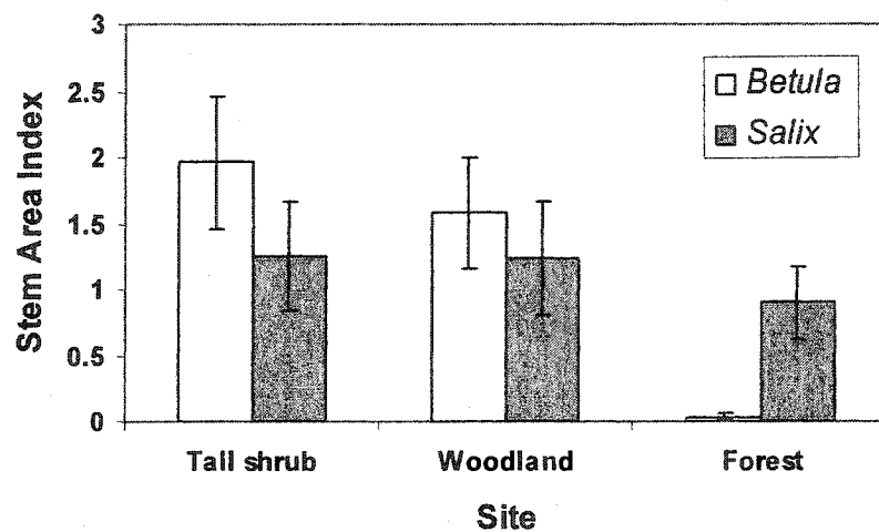
Figure 2.4: Betula and Salix Stem Area Index (SAI) for the sites with a tall shrub component to the canopy. Mean and standard error shown. Units for SAI are \text{m}^2/\text{m}^2 .
