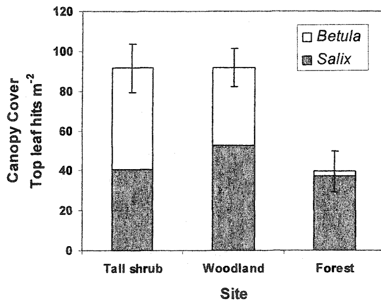
Figure 2.2: Canopy cover of Betula and Salix shrubs measured with a point frame. Hits on the top leaf of each species determine canopy cover. Data shown are mean and standard error.
