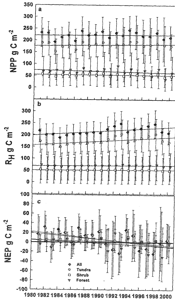
Figure 3.2: NPP, RH and NEP fluxes for the domain. Mean and standard deviation shown for combined vegetation and tundra, shrub and forest results separately.
