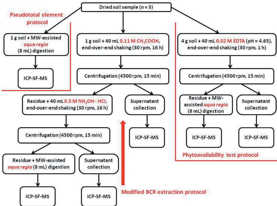
Figure 1. Schematic diagram of the sample preparation steps and analysis performed on the investigated soil samples. BCR = Community Bureau of Reference, European Commission.
