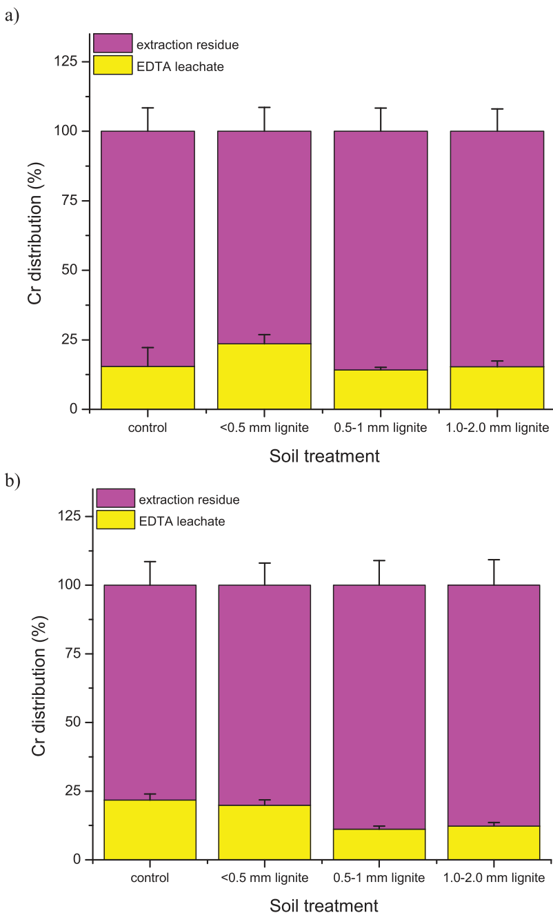
Figure 6. Chromium distribution (%) between the EDTA leachates and extraction residue of calcareous (a) and acidic (b) sandy soils without lignite or containing 5.0% lignite by weight and particle size ranges of <0.5 mm; 0.5–1.0 mm or 1.0–2.0 mm after eight weeks of incubation with 375 mg/kg Cr(III). Residual percentage originates from individual measurements.
