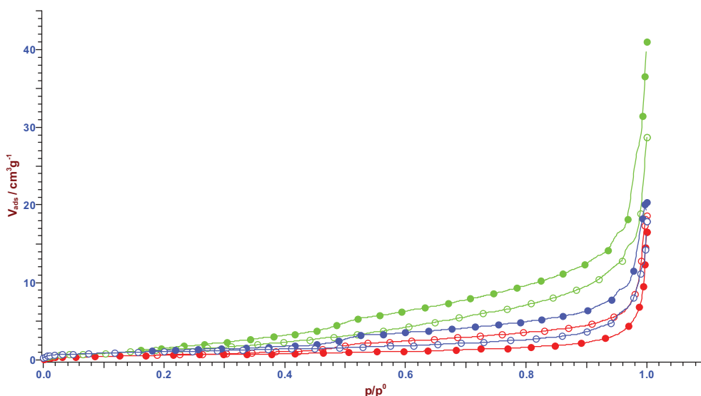
Figure 3. Nitrogen gas adsorption-desorption isotherms of the studied lignite samples as a function of particle size: 1.0–2.0 mm (red); 0.5–1.0 mm (blue) and <0.5 mm (green). Symbols of filled and empty circles were used to indicate adsorption and desorption isotherms, respectively.
