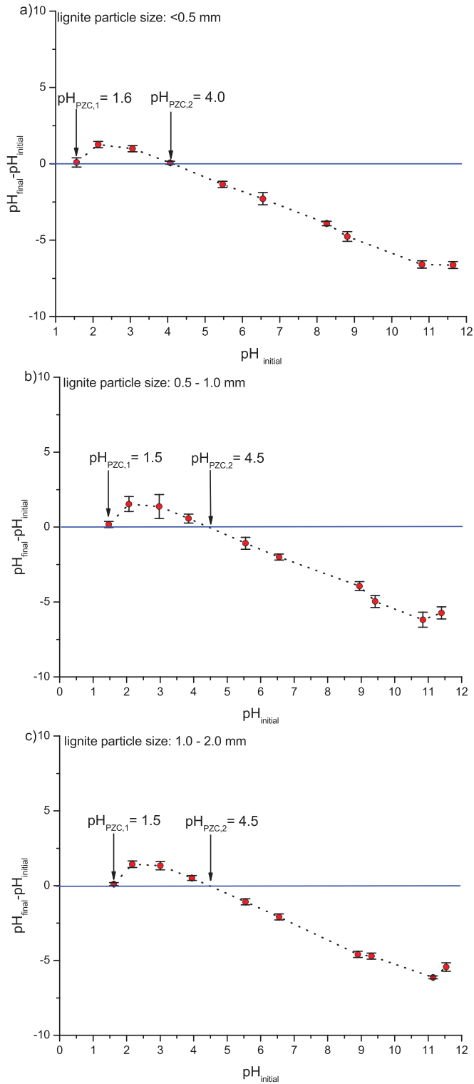
Figure 4. Point of zero charge (PZC \pm standard deviation) values ( n = 3 ) of lignite having <0.5 mm (a); 0.5–1.0 mm (b) and 1.0–2.0 mm (c) particle size ranges determined by the pH drift method. Data were connected with dashed lines for better visualization of the PZC values.
