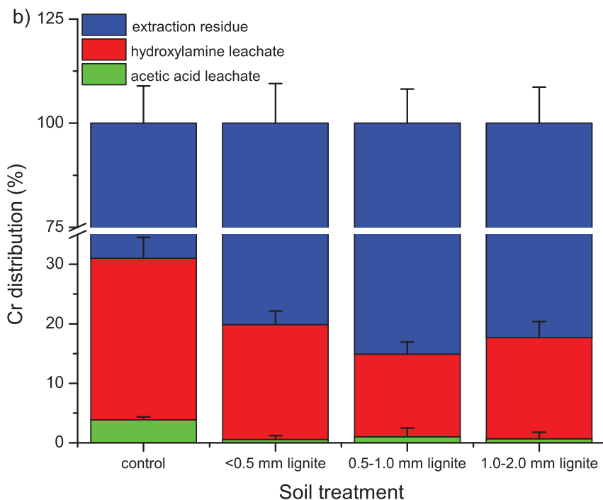
Figure 5. Chromium distribution (%) among different leachates of calcareous (a) and acidic (b) sandy soils without lignite or containing 5.0% lignite by weight and particle size ranges of <0.5 mm; 0.5–1.0 mm or 1.0–2.0 mm after eight weeks of incubation with 375 mg/kg Cr(III). Residual percentage originated from individual measurements.
