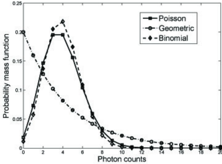
Fig. 2. This figure shows Poisson, geometric and binomial probability mass functions. The various parameters used are \lambda = 4 for Poisson, p = 0.2 for geometric, and n = 20, p = 0.2 for binomial. In all three cases the mean value is 4.
