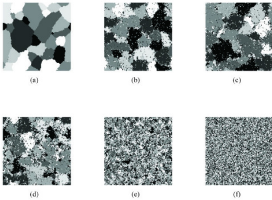
Fig. 9. Sample MRF images generated according to a generalized Ising model with potential energies given by (18) using various values for the parameter \beta . We employed a Metropolis sampler using 1000 iterations. The values used for the parameter \beta are (a) \beta = -2 , (b) \beta = -1 , (c) \beta = -0.975 , (d) \beta = -0.95 , and (e) \beta = -0.9 , (f) \beta = -0.4 .
