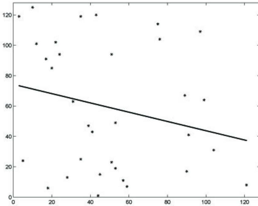
Fig. 3. Figure showing the output 128x128 photon-counted array, where the photon counts are represented by the symbols ‘*’, and the best-fit estimate of the line from the photon counts. The value of k is 5 and the corresponding noise variance is 2.08. Here N_p \epsilon = 0.3 .
