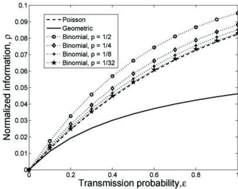
Fig. 6. Normalized mutual information for different possible channel distributions while using a Markov-chain model for P_{\mathbf{x}(\mathbf{x})} , with a specific correlation index, m = 0.01 . Here we used N_p = 3 .
