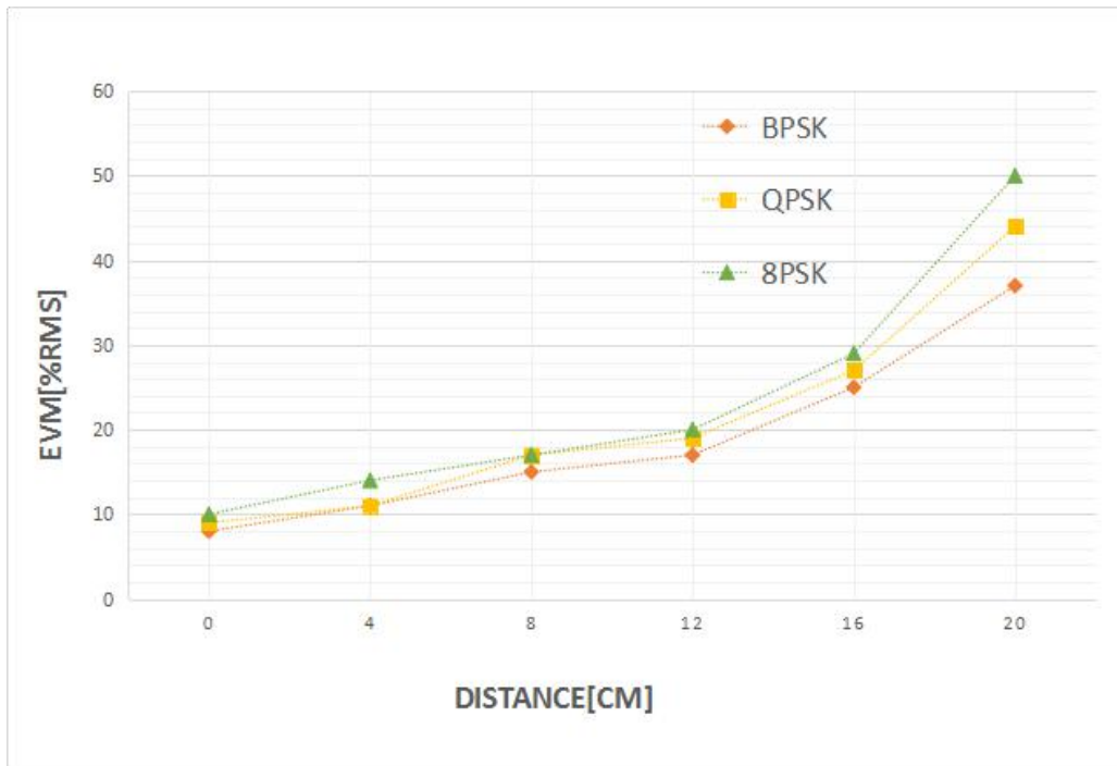
Figure21. Distance and EVM (PSK)
