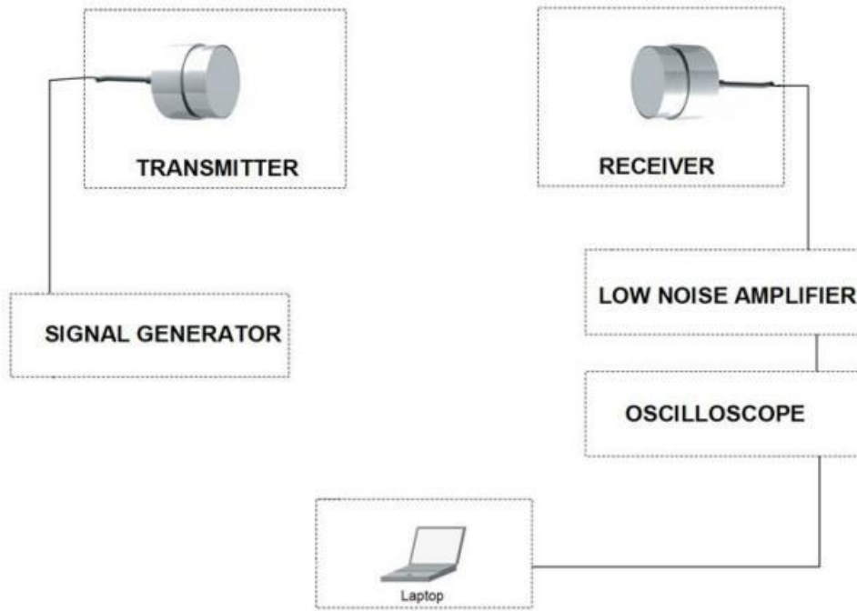
Figure6. Setup of Low-Frequency Communication
