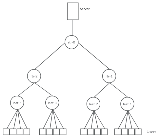
FIGURE 3.2: Tree Topology.
