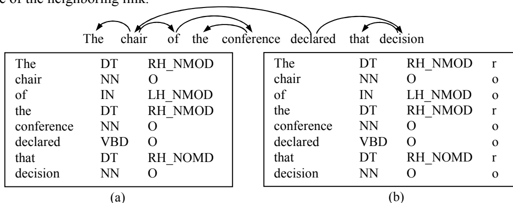
Figure 1: Example of (a) the sequential neighboring relation labeling, (b) the reduce decision labeling.
