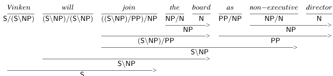
Figure 1: CCG derivation: lexical categories (the interest of this paper) appear below words and derived categories appear below lines showing combination using the forward application rule ( X/Y Y \rightarrow X ).
