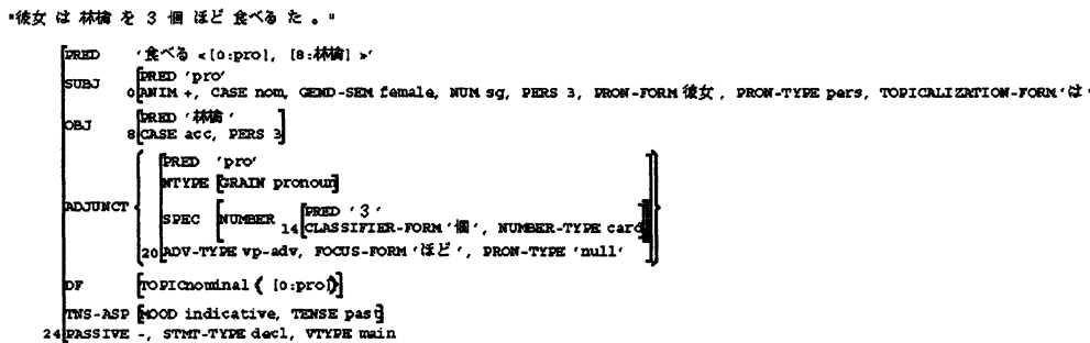
Figure 6: f-structure for (3)
