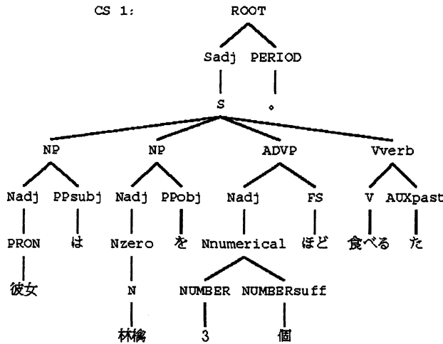
Figure 5: c-structure for (3)
