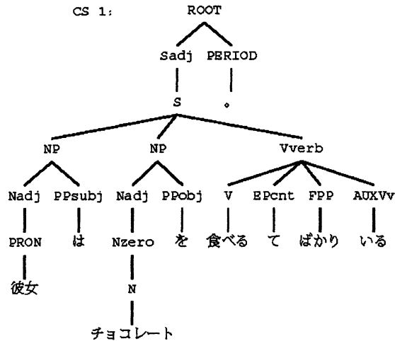
Figure 7: c-structure for (6)
