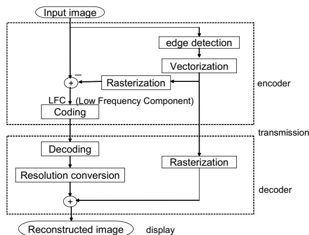
Fig. 1. Flow of proposed method
