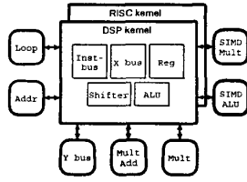
Figure 1. Processor kernels and hardware units.
