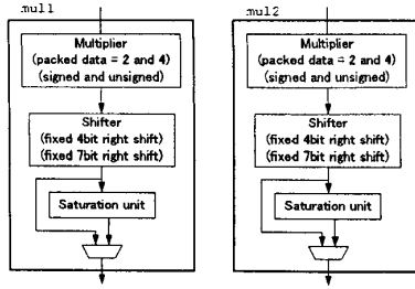
Figure 5. Original multiplier configuration.
