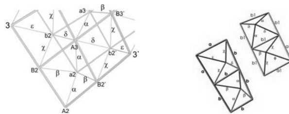
Figure 23a Types of struts – diagonals of rotating hyperbolic cylinder
