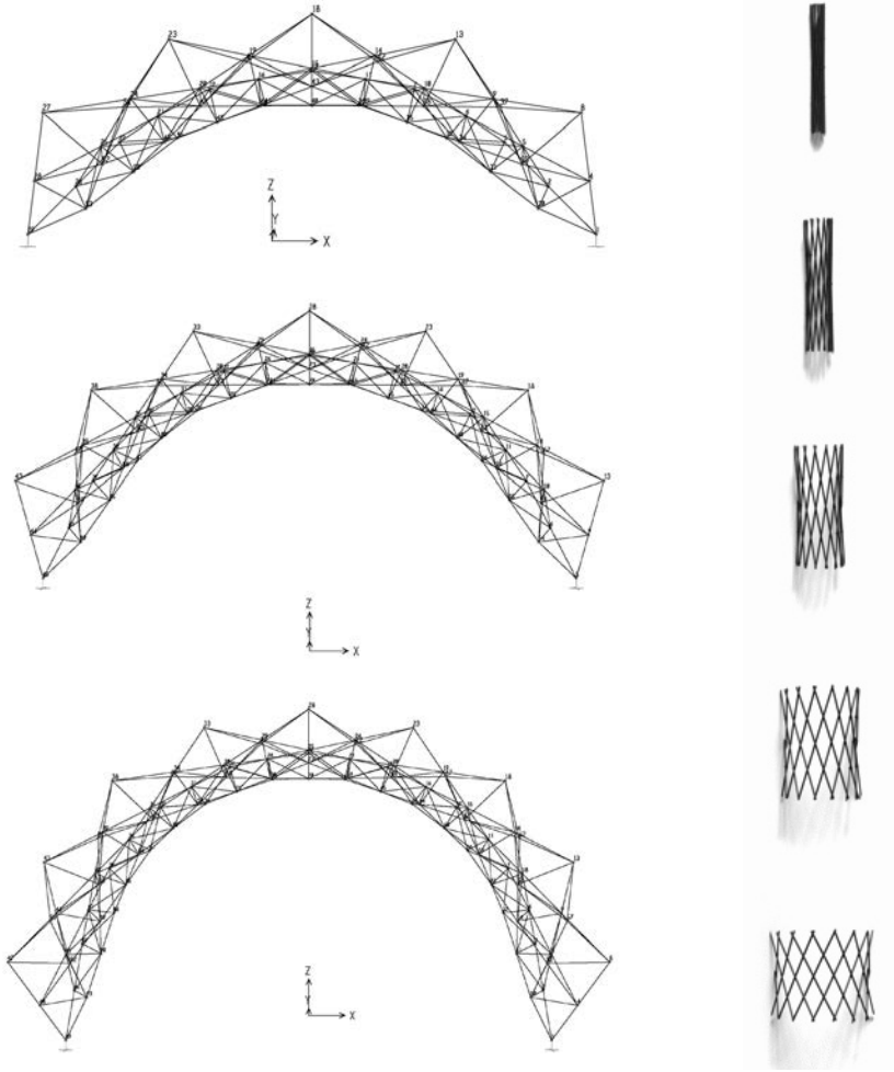
Figure 25 Static characteristics of the structure
