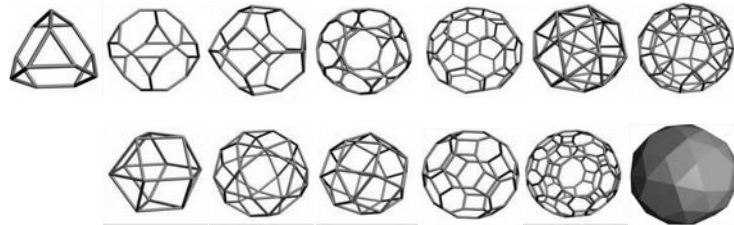
Figure 2 Archimedean solids
