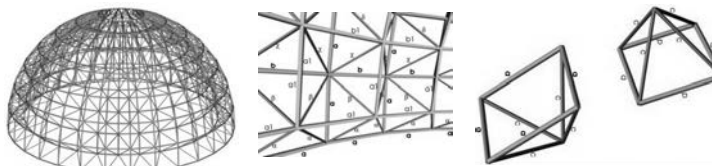
Figure 18 Space grid geometric shape of the calotte
