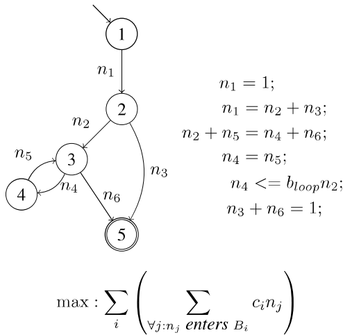
Figure 2. Control flow graph and the corresponding flow constraints
