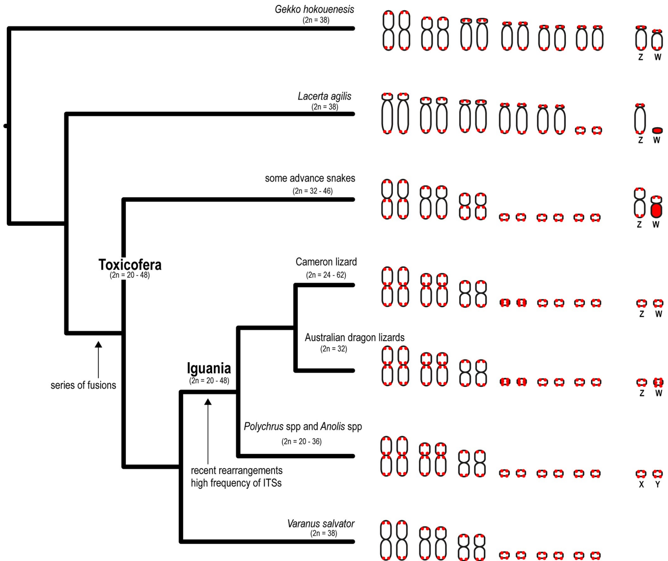
Fig 4. Schematic representation of the distribution of interstitial telomeric sites (ITSs) in centromeric or pericentromeric regions on chromosomes and amplification of telomeric repeats on sex chromosome in lizards and snakes. Phylogeny was partially derived from Pyron et al. [39]. Distribution of ITSs and telomeric repeat amplifications of lizards and snakes were also obtained from Young et al. [11], Matsubara et al. [37], Augstenová et al. [34], Rovatsos et al. [23,30] and Srikulnath et al. [7,9].
