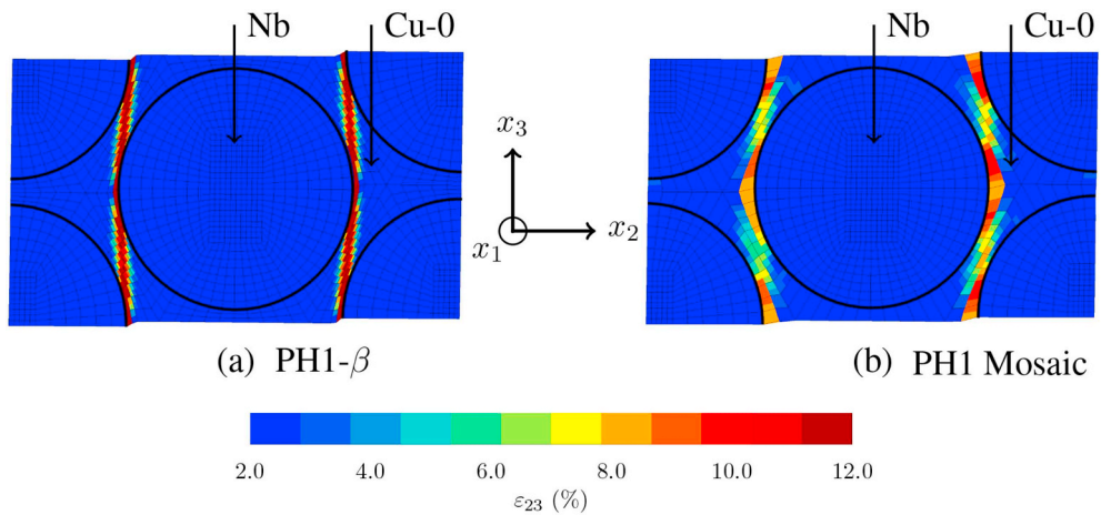
Fig. 12. Shear strain \varepsilon_{23} distribution predicted by the (a) PH1- \beta and (b) PH1 Mosaic models at scale H1 with an overall effective transverse shear (\bar{\varepsilon}_{23})_{H1} = 1.5\% imposed in the TS test.
