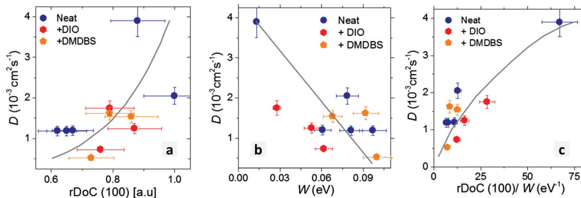
Fig. 7 Dependence of exciton diffusion coefficient D in P3HT-co-P3DDT films on a relative degree of crystallinity r\text{DoC}(100) (a); free exciton bandwidth W (b); and on the ratio of r\text{DoC}(100) and W (c). Films were spin-coated from neat solutions or with additives as indicated in the legend. Data points at D = 3.9 \times 10^{-3} \text{ cm}^2 \text{ s}^{-1} which give one-dimensional diffusion length of 10 nm correspond to the solvent-vapour annealed thin film. Solid lines are guides to eye only.
