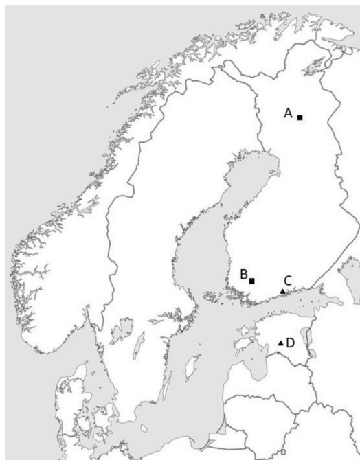
Fig. 1. Location of the paired sites (▲ – only chamber measurements, ■ – EC measurements in pristine sites in addition to chamber measurements). A) Sodankylä, B) Tammela, C) Sipoo, D) Viljandi.
