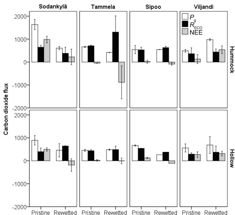
Fig. 4. Modelled gross photosynthesis ( P_g ), ecosystem respiration ( R_{ECO} ), and net ecosystem exchange (NEE) (g CO 2 m -2 ) ( \pm SE) for the period from May–September 2015 based on chamber measurements. NEE = P_g - R_{ECO} . Note that P_g and R_{ECO} are always positive for clarity. Therefore, NEE is positive if the ecosystem is a CO 2 sink during the growing season while NEE is negative if the ecosystem is a CO 2 source during the growing season.
