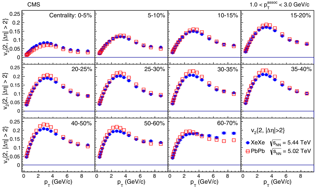
FIG. 6. Comparison of the v_2 results measured with two-particle correlations from two different systems, XeXe collisions at \sqrt{s_{NN}} = 5.44 TeV and PbPb collisions at 5.02 TeV, shown as a function of p_T in eleven centrality bins. The bars (smaller than the marker size) and the shaded boxes represent statistical and systematic uncertainties, respectively.
