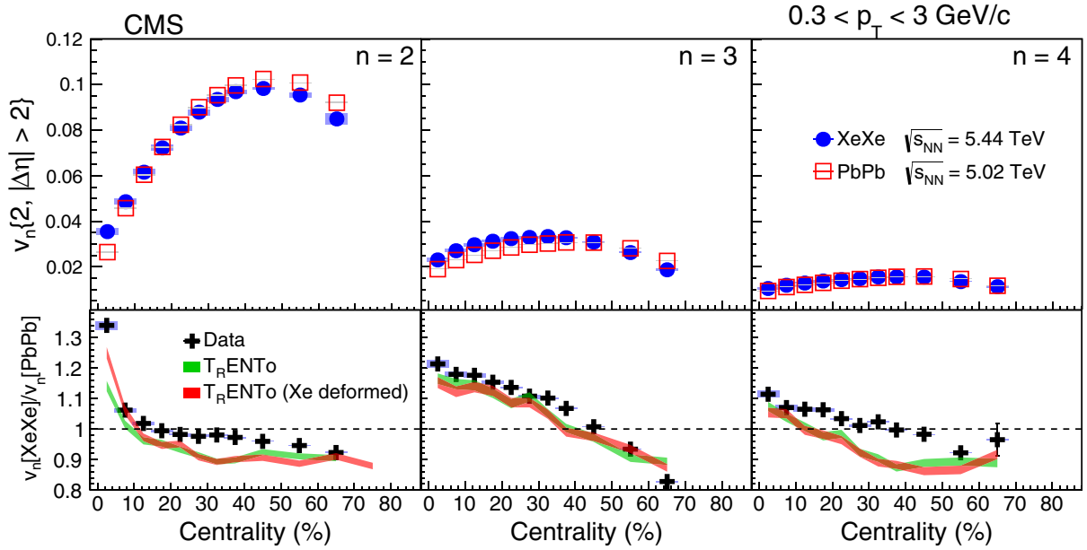
FIG. 10. Centrality dependence of the spectrum-weighted v_2 , v_3 , and v_4 harmonic coefficients from two-particle correlations method for 0.3 < p_T < 3.0 GeV/c for XeXe collisions at \sqrt{s_{NN}} = 5.44 TeV and PbPb collisions at 5.02 TeV. The lower panels show the ratio of the results for the two systems. The bars and the shaded boxes represent statistical and systematic uncertainties, respectively. Theoretical predictions from Ref. [37] are compared to the data (shaded bands). The model calculation is done for the p_T range 0.2 < p_T < 5.0 GeV/c.
