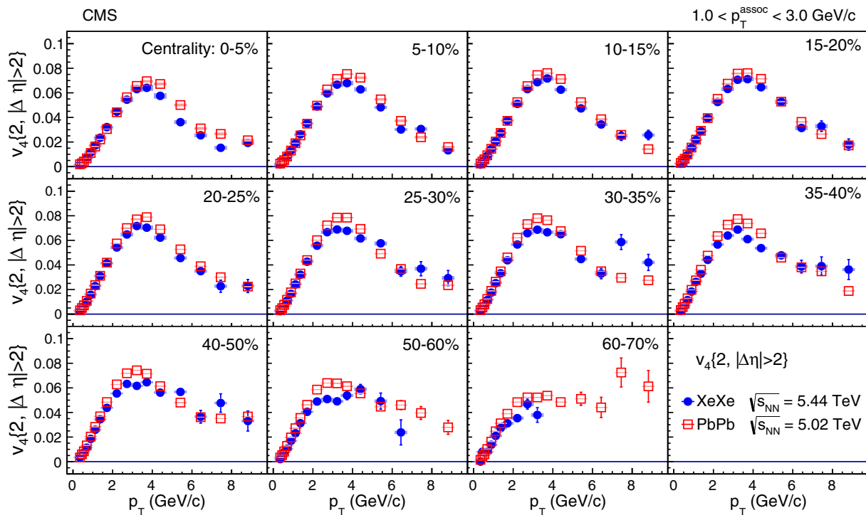
FIG. 8. Comparison of the v_4 results measured with two-particle correlations from two different systems, XeXe collisions at \sqrt{s_{NN}} = 5.44 TeV and PbPb collisions at 5.02 TeV, shown as a function of p_T in 11 centrality bins. The bars and the shaded boxes represent statistical and systematic uncertainties, respectively.
