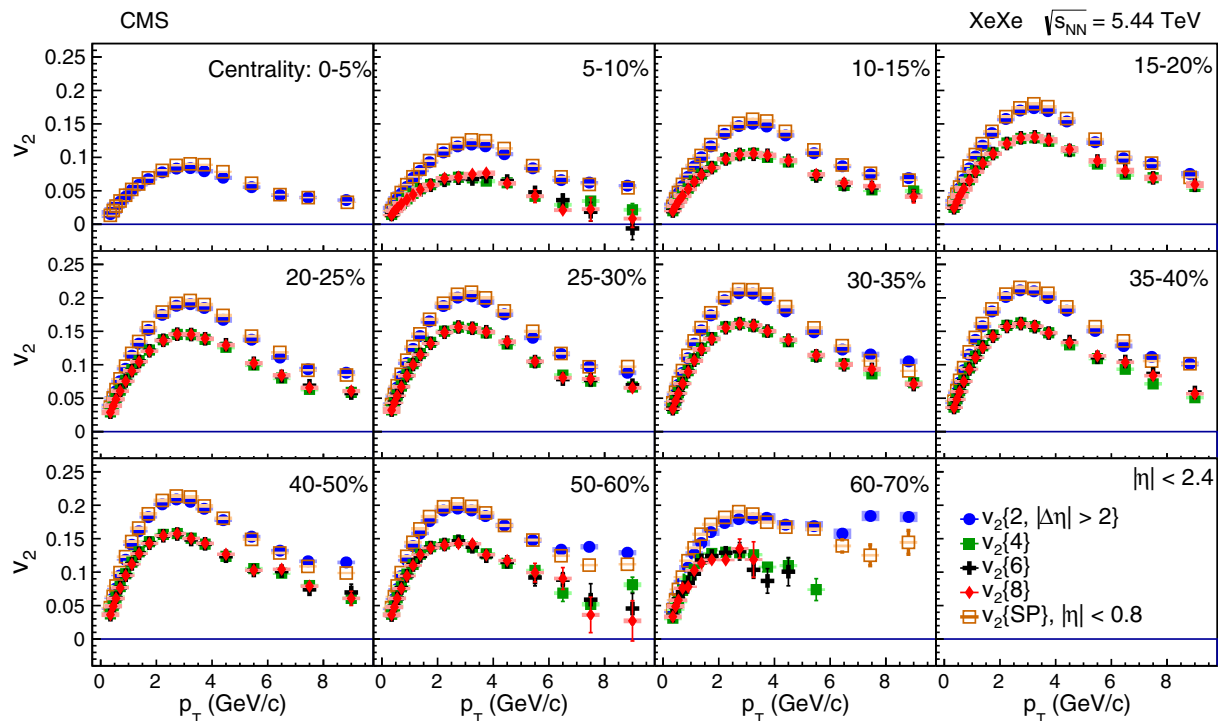
FIG. 1. Elliptic-flow coefficients v_2 based on different analysis techniques, as functions of transverse momentum and in bins of centrality, from the 5% most central (top left) to 60–70% centrality (bottom right). The results for the two-particle and multiparticle correlations correspond to the range |\eta| < 2.4 , while the scalar-product results are for |\eta| < 0.8 . The bars and the shaded boxes represent statistical and systematic uncertainties, respectively.
