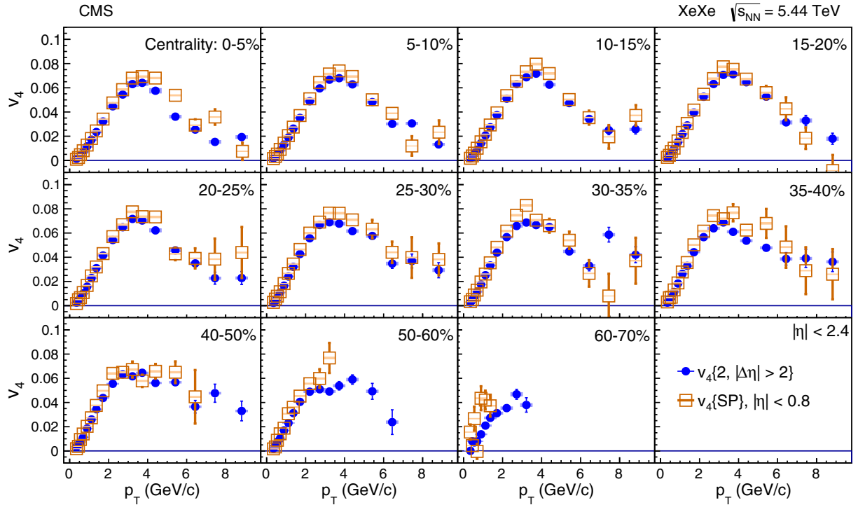
FIG. 3. The v_4 coefficients, based on the different analysis techniques, as functions of transverse momentum and in bins of centrality, from the 5% most central (top left) to 60–70% centrality (bottom right). The results for the two-particle correlations correspond to the range |\eta| < 2.4 , while the scalar-product results are for |\eta| < 0.8 . The bars and the shaded boxes represent statistical and systematic uncertainties, respectively.
