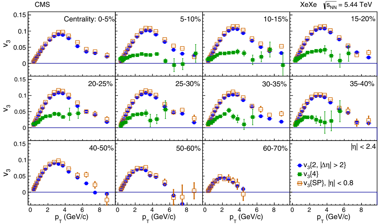
FIG. 2. Triangular-flow coefficients v_3 based on the different analysis techniques, as functions of transverse momentum and in bins of centrality, from the 5% most central (top left) to 60–70% centrality (bottom right). The results for the two-particle and multiparticle correlations correspond to the range |\eta| < 2.4 , while the scalar-product results are for |\eta| < 0.8 . The bars and the shaded boxes represent statistical and systematic uncertainties, respectively.
