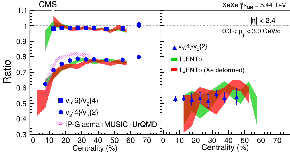
FIG. 5. Centrality dependence of v_2\{4\}/v_2\{2\} , v_2\{6\}/v_2\{4\} (left panel), and v_3\{4\}/v_3\{2\} (right panel) ratios. The shaded bands represent the theoretical predictions based on the IP-GLASMA+MUSIC+UrQMD and the relativistic hydrodynamic model from Ref. [37] considering both spherical and deformed xenon nuclei, while the widths of the areas show the statistical uncertainties of the model. The T_R ENTo calculation is done for the p_T range 0.2 < p_T < 5.0 GeV/c.
