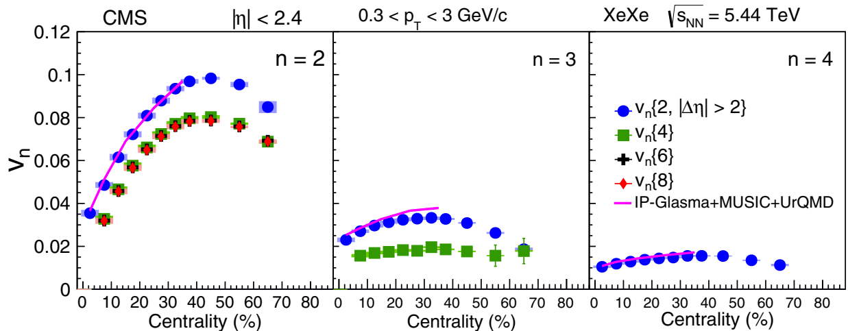
FIG. 4. Centrality dependence of the spectrum-weighted v_2 , v_3 , and v_4 flow harmonics with 0.3 < p_T < 3.0 GeV/c. The v_2 results are shown for two-, four-, six-, and eight-particle correlations (left panel). The v_3 results are shown for two- and four-particle correlations (middle panel), while the v_4 values are presented for two-particle correlations technique, only. The solid curve in each panel is the IP-GLASMA+MUSIC+UrQMD prediction for v_n\{2\} . The shaded boxes represent systematic uncertainties.
