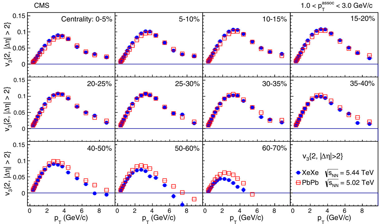
FIG. 7. Comparison of the v_3 results measured with two-particle correlations from two different systems, XeXe collisions at \sqrt{s_{NN}} = 5.44 TeV and PbPb collisions at 5.02 TeV, shown as a function of p_T in 11 centrality bins. The bars (smaller than the marker size) and the shaded boxes represent statistical and systematic uncertainties, respectively.
