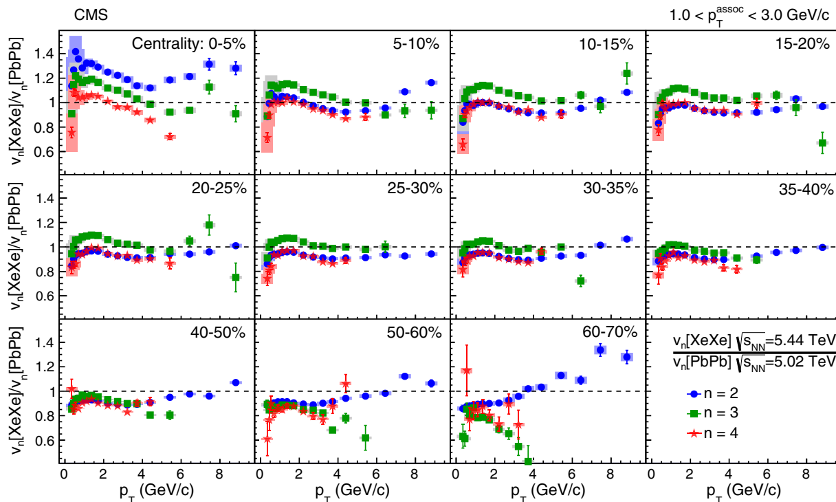
FIG. 9. Ratios of the v_2 , v_3 , and v_4 harmonic coefficients from two-particle correlations in XeXe and PbPb collisions as functions of p_T in 11 centrality bins. The bars and the shaded boxes represent statistical and systematic uncertainties, respectively.
