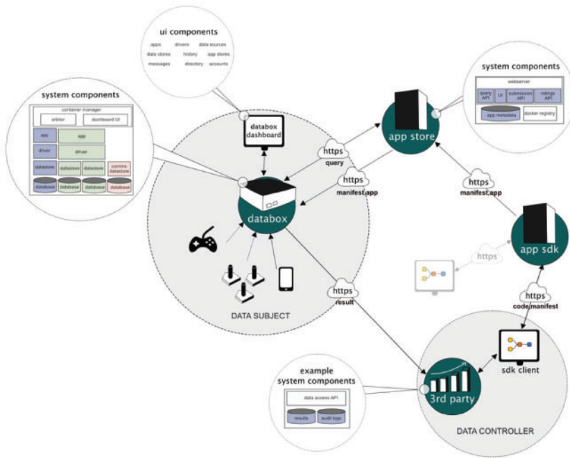
Figure 1: The IoT Databox model.
