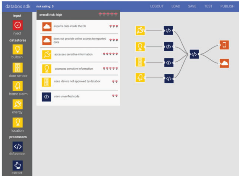
Figure 4: The SDK: risk-rating apps during their development.
