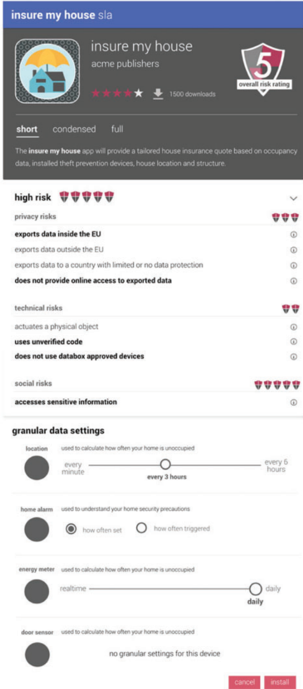
Figure 2: Enabling granular choice.
