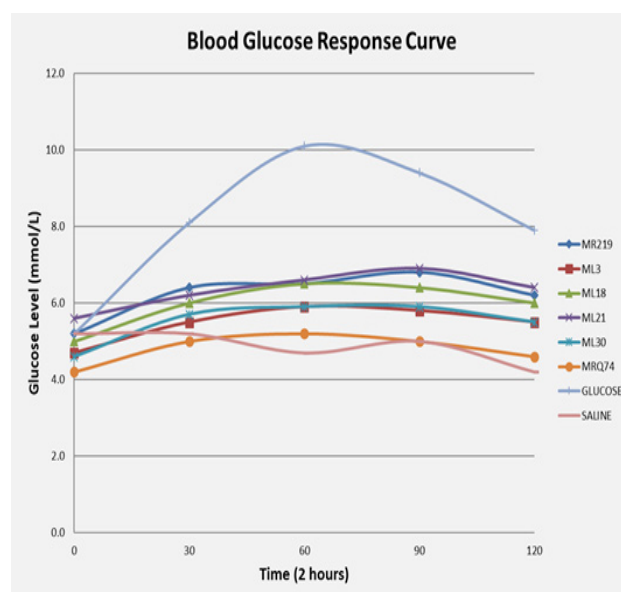
Figure 1. Blood glucose response curves of tested foods at 30 minutes intervals.
