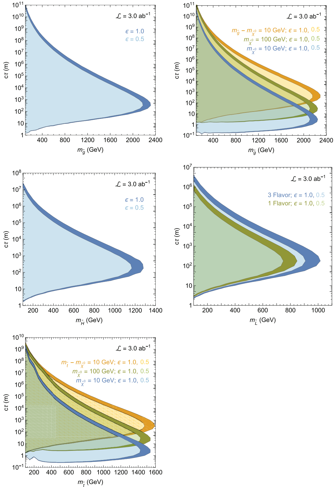
Figure 15. Projected MATHUSLA reach (assuming the 200 m × 200 m × 20 m benchmark geometry of figure 1) for several LSP and production scenarios with 3 ab -1 . We assume that the decay of the LSP leads to visible particles in the MATHUSLA detector. In order: direct gluino pair-production, prompt gluino pair decay to long-lived bins (for discrete bino mass choices), direct Higgsino pair-production, direct sneutrino pair-production, and prompt stop pair decays to long-lived bins (for discrete bino mass choices). The efficiency is varied from 0.5-1 (darker bands) in order to take into account the difference in efficiencies for each particular LSP decay mode.
