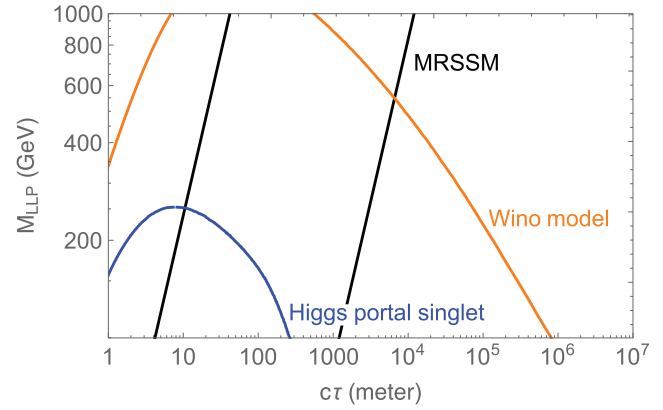
Figure 35. MATHUSLA reach for the models described in section 6.1.3 for long-lived particle masses M_{LLP} = 0.1 –1 TeV and decay lengths c\tau > m for 14 TeV HL-LHC, computed using the analytical approximations outlined in section 3.1.1. (Regions between the solid lines give N_{obs} > 4 in MATHUSLA.) Note that these models give successful baryogenesis inside the full parameter space shown. The MRSSM reach projection assumes Bino LLP production in the decay of a 1.8 TeV gluino. The Higgs portal singlet projection is shown for c_H v / \Lambda_H = 0.5 . This estimate assumes the 200 \text{ m} \times 200 \text{ m} \times 20 \text{ m} benchmark geometry of figure 1.
