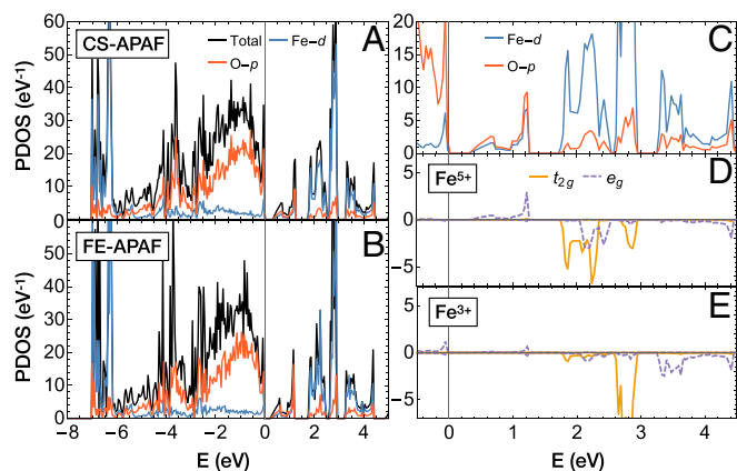
Fig. 4. Total density of states (black line) and orbital PDOS for Fe- d (blue) and O- p (red) orbitals of CS-APAF (A) and FE-APAF (B) phases. (C) Close-up of PDOS for the unoccupied states. (D) PDOS of unoccupied t_{2g} and e_g states for the spin-up \text{Fe}^{5+} site. (E) PDOS of unoccupied t_{2g} and e_g states for the spin-up \text{Fe}^{3+} site.
