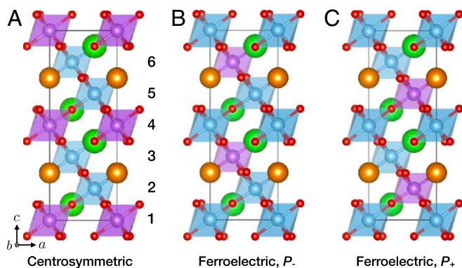
Fig. 3. Three charge-ordering patterns for A-cation ordered superlattices. (A) Centrosymmetric charge-ordering pattern. (B and C) Ferroelectric charge-ordering patterns with 2 polar variants in which P_+/P_- are related by inversion. The Fe layers are numbered 1 to 6. For both the centrosymmetric and the ferroelectric phases, the c -axis rotations of the octahedra in layers 1, 2, and 3 are opposite to those in layers 4, 5, and 6, respectively.
