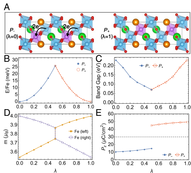
Fig. 5. (A) Atomic arrangements of 2 inversion-related polar variants, P_- and P_+ , showing the electron transfer relating the two. (B) Total energy per Fe for atomic arrangements linearly interpolated between those of the 2 polar variants shown in A. The zero of energy is taken as the energy of the 2 polar variants. \lambda is the interpolation parameter ranging from \lambda=0 for P_- to \lambda=1 for P_+ . (C) \lambda dependence of the DFT+U band gap. (D) \lambda dependence of the magnetic moments of the 2 Fe sites adjacent to the La layer (A, Left and Right). (E) \lambda dependence of the polarization parallel to the c axis assuming a branch choice corresponding to the electron transfer in A. The dashed line is drawn at half the quantum of polarization, for reference.
