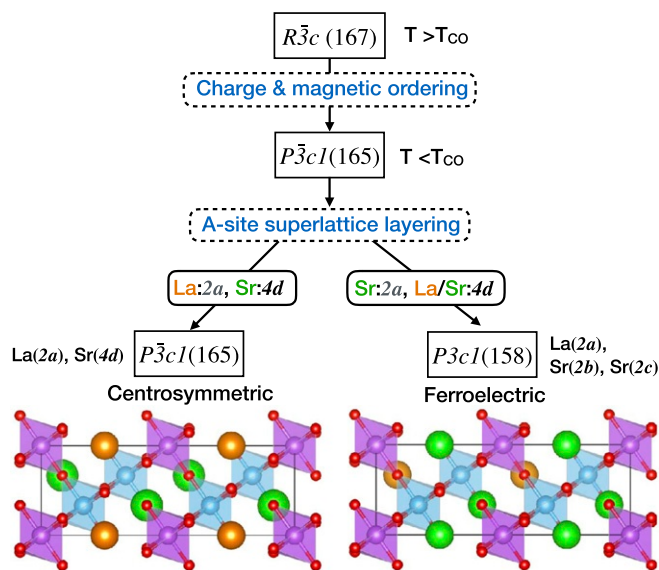
Fig. 2. Space group analysis of symmetry lowering in the LSFO solid solution. Starting from the high-temperature R\bar{3}c structure, the charge ordering lowers the symmetry to the P\bar{3}c1 space group. From there, different superlattice layering arrangements described in the text produce centrosymmetric and ferroelectric phases.
