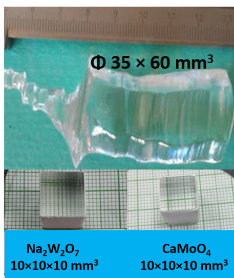
Fig. 1 Photographic views of grown NWO crystal and measured samples of NWO and CMO crystals
