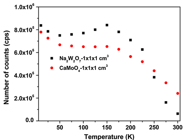
Fig. 8 Temperature dependent scintillation light yield comparison of NWO and CMO crystals using ^{90}\text{Sr} beta source as the excitation source
