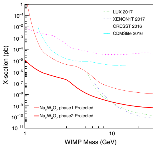
Fig. 10 Expected 90% confidence level limits on the WIMP-nucleon spin-independent (SI) cross section with NWO crystals are presented. Thin red solid line represents a case of 10kg NWO crystal, 1 counts/keV/kg/day background, and 1keV energy threshold and thick red solid line corresponds to a case of 50kg crystal, 0.1 counts/keV/kg/day background, and 0.5keV energy threshold
