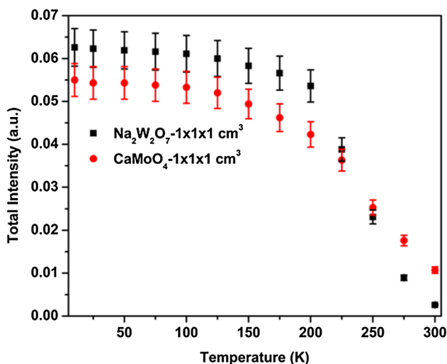
Fig. 7 Luminescence light yields comparison of NWO and CMO crystal at different temperatures, using a 280-nm-wavelength LED excitation source
