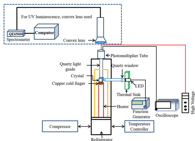
Fig. 2 A Schematic diagram of the low temperature setup for luminescence decay time and light yield measurement
