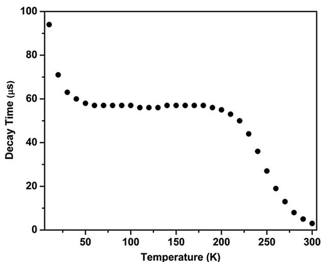
Fig. 6 Decay constants of a NWO crystal as a function of temperature
