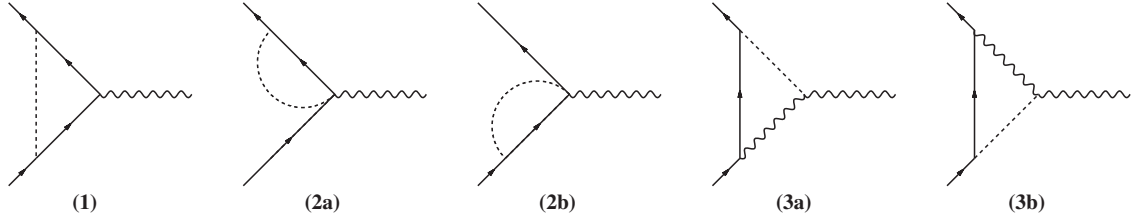
FIG. 1. Graviton contributions at one loop to the anomalous magnetic moment of muon. The dashed lines denote gravitons and the curly lines are photons.
