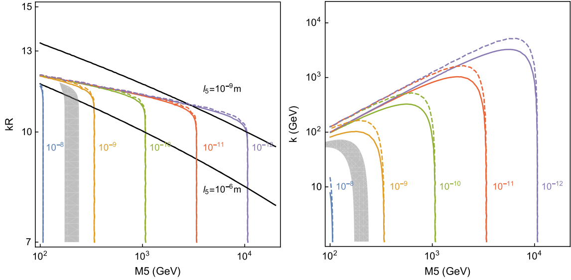
FIG. 4. The contribution of the KK gravitons to the muon g-2 for \Delta a_\mu = 10^{-8}, \dots, 10^{-12} in the M_5 - kR (left) and M_5 - k (right) plots. The contributions from the clockwork gravitons are shown by the solid lines. Here we also show the contributions with the Randall-Sundrum background, Eq. (31), by dashed lines. The gray region is the 1\sigma band of the current muon g-2 anomaly [16]. In the left panel, the size of extra dimension, l_5 [Eq. (26)] is shown by black lines for l_5 = 10^{-6} m and 10^{-9} m.
