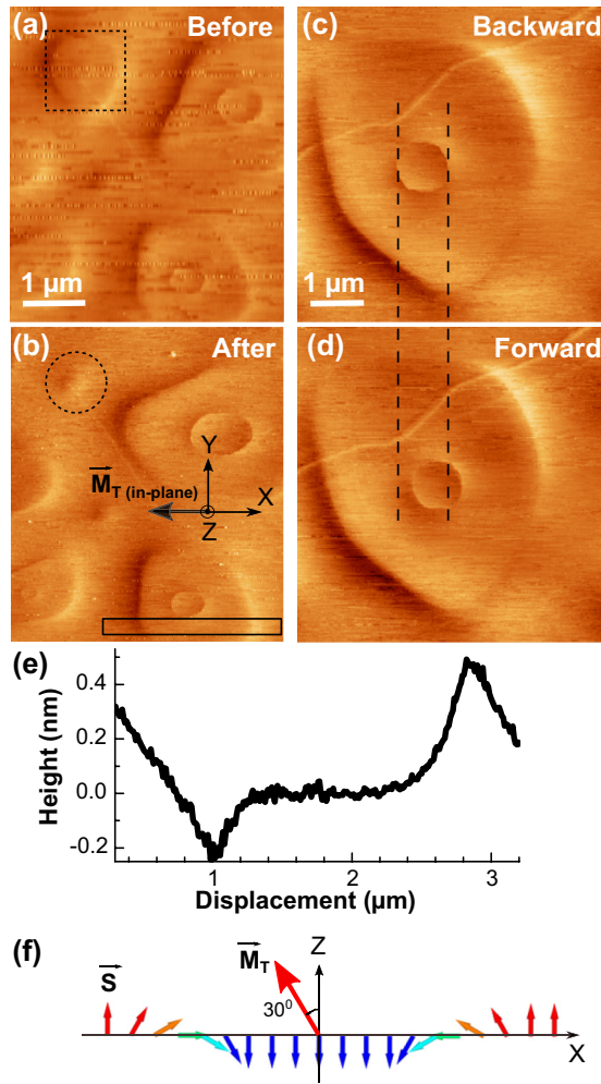
FIG. 3. (a, b) STM images of magnetic domains before (a) and after (b) tip-induced conversion of a double-walled domain (marked with dashed black box) into a bubble domain (marked with dashed black circle). (c, d) STM images of a double-walled domain showing a displacement of the inner wall between the backward (c) and the forward (d) scanned images, while the outer domain wall stays the same (sample bias V_s = -0.5 V, tunneling current I = 100 pA, temperature T = 120 K). (e) Line profile across the outer walls of double-walled domain along the rectangle in (b). (f) Schematic spin structure of a Neel domain wall with respect to the STM tip magnetization \vec{M}_T .
