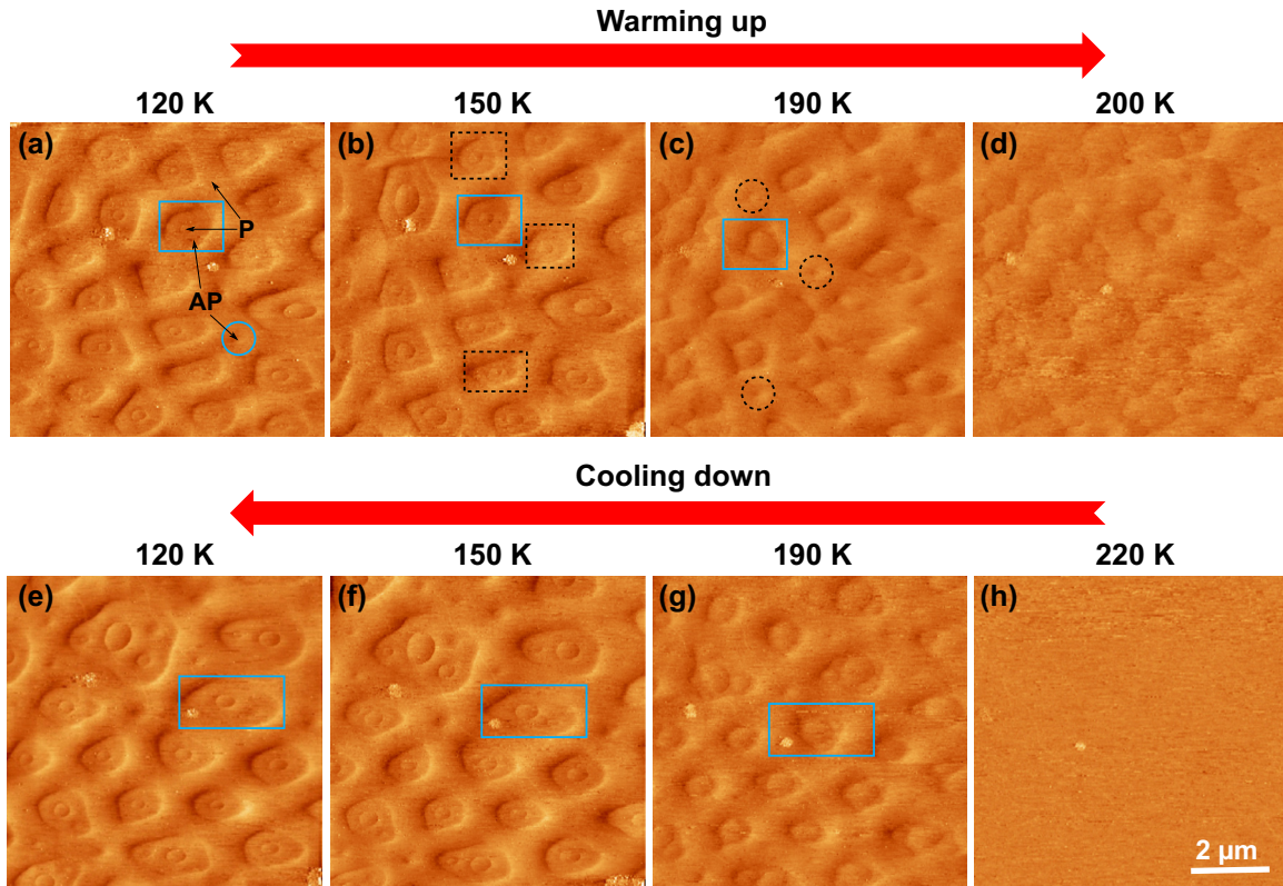
FIG. 2. The evolution of the FC magnetic domains through varying sample temperatures between 120 and 220 K. The magnetic domains were induced by keeping the Ni tip 3 \mu\text{m} away from the surface when cooling the sample down from the room temperature. The Ni tip is kept 1 \mu\text{m} away from the surface at the image corner during warming up (a–d) and cooling down (h–e). The scanning parameters are kept the same of sample bias V_s = -0.5 \text{ V} , tunneling current I = 50 \text{ pA} . The blue box and circle in (a) mark an example of a double-walled domain and a bubble domain, respectively. P and AP point to the domain areas with the magnetization parallel (P) and antiparallel (AP) to the tip magnetization. The dashed black circles in (c) mark the bubble domains newly converted from double-walled domains [marked by dashed black boxes in (b)] during warming from 150 to 190 K.
