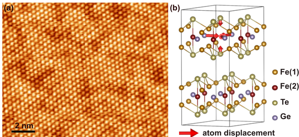
FIG. 5. (a) Atomically resolved STM image acquired with a W tip on cleaved \text{Fe}_3\text{GeTe}_2 ( V_s = -0.5 V, I = 100 pA, T = 120 K). (b) Density functional theory results showing atomic displacements (indicated by red arrows) induced by an Fe(2) vacancy in a \sqrt{3} \times \sqrt{3} supercell.
