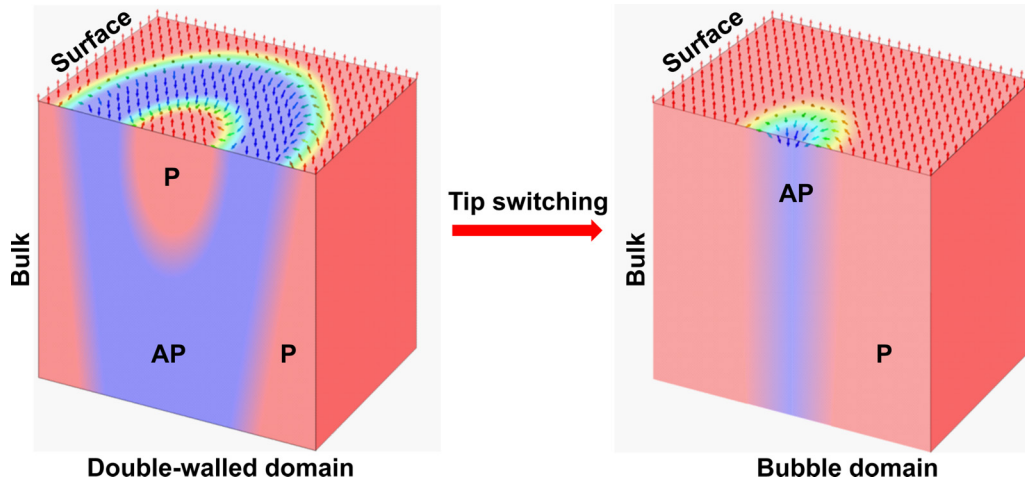
FIG. 6. The schematic micromagnetic domain structure of the FC double-walled domain and bubble domain. The blue and red colors represent two opposite magnetization directions which are antiparallel (blue) and parallel (red) to the tip magnetization, respectively.
