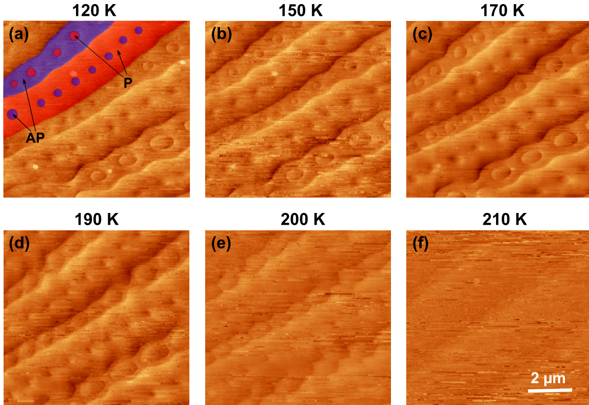
FIG. 1. The evolution of ZFC magnetic domains of cleaved \text{Fe}_3\text{GeTe}_2 visualized by STM imaging with a Ni tip while increasing sample temperature from 120 to 210 K. The semitransparent overlays in (a) illustrate the magnetizations parallel (P, red color) and antiparallel (AP, blue color) to the tip magnetization. The Ni tip is kept 10 mm away from the surface when cooling from the room temperature to 120 K to avoid the effect of Ni tip stray field on the formation of the magnetic domains. During warming up, the Ni is kept 1 \mu\text{m} away from the surface at the image corner. The scanning parameters are kept the same: V_s = -0.5 \text{ V} , I = 50 \text{ pA} .
