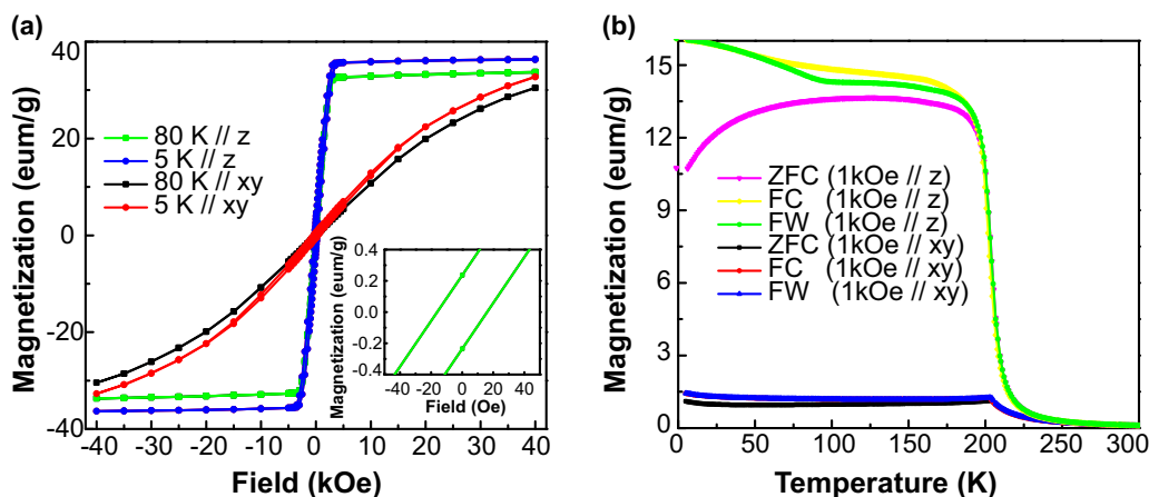
FIG. 4. (a) Field-dependent magnetization plot at 80 and 5 K. The external field is applied in H \parallel xy and H \parallel z directions, respectively. Inset is the zoom-in section showing coercive field for \text{Fe}_3\text{GeTe}_2 at 80 K. (b) Magnetization as a function of temperature. The applied field (1 kOe) is in H \parallel xy and H \parallel z .
