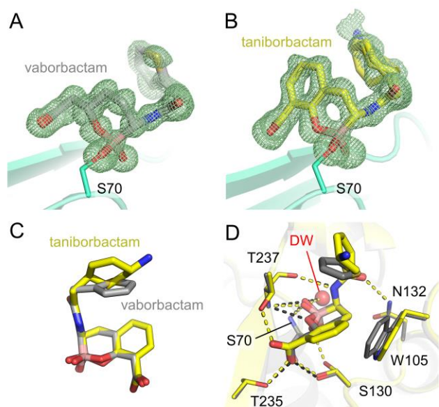
Figure 2. Views from crystal structures of cyclic boronate binding to KPC-2.
