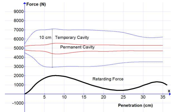
Figure 1. Retarding force, temporary cavity, and permanent cavity of the Lehigh Defense Maximum Expansion bullet impacting ballistic gelatin at 830 ft/s (253 m/s) with 306 ft lbs (415 Nm) of kinetic energy.
