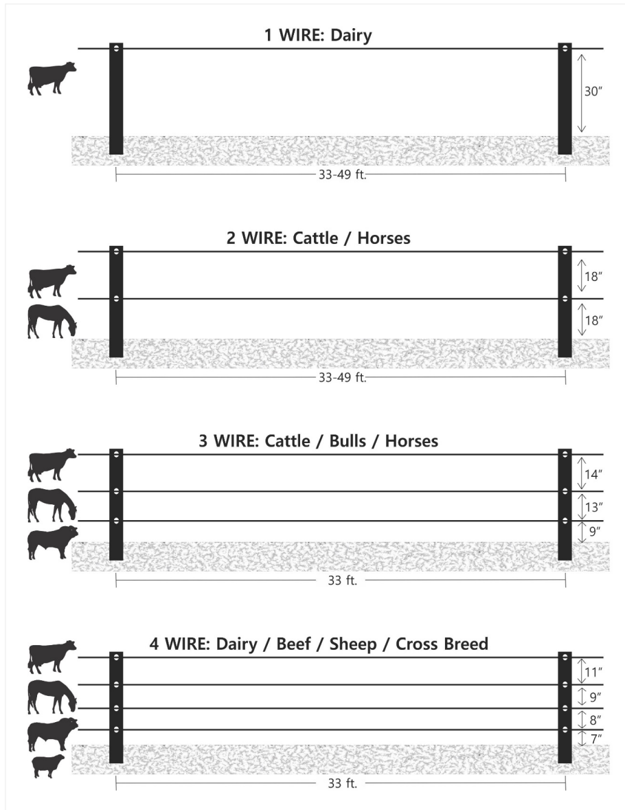
Figure 2: Ideal wire spacing for livestock (Staffix, n.d.).
