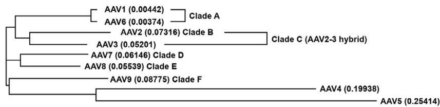
Figure 2. Phylogenetic Relationships among AAV Serotypes
