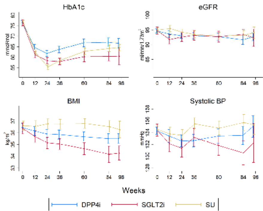
Figure 2. Mean (95% confidence intervals) of each clinical measure during treatment, for propensity score matched cohorts of individuals following intensification with DPP4i, SGLT2i and SU after metformin monotherapy.
