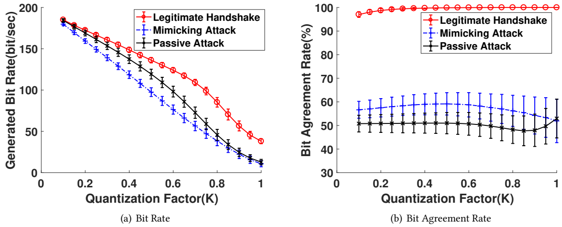
Fig. 9. The impact of different quantization factor ( K ) on the system performance in terms of (a) bit rate, (b) bit agreement rate
