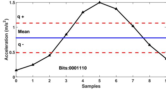
Fig. 5. Illustration of quantization process we use to generate bits stream, figure was first presented in our previous work [31]
