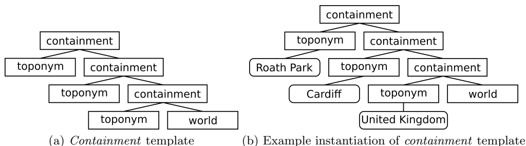
Fig. 10. Containment templates. a) The structure of the containment template. b) Example instantiation of the containment template, which would be realised with the phrase “in Roath Park, Cardiff, United Kingdom”
