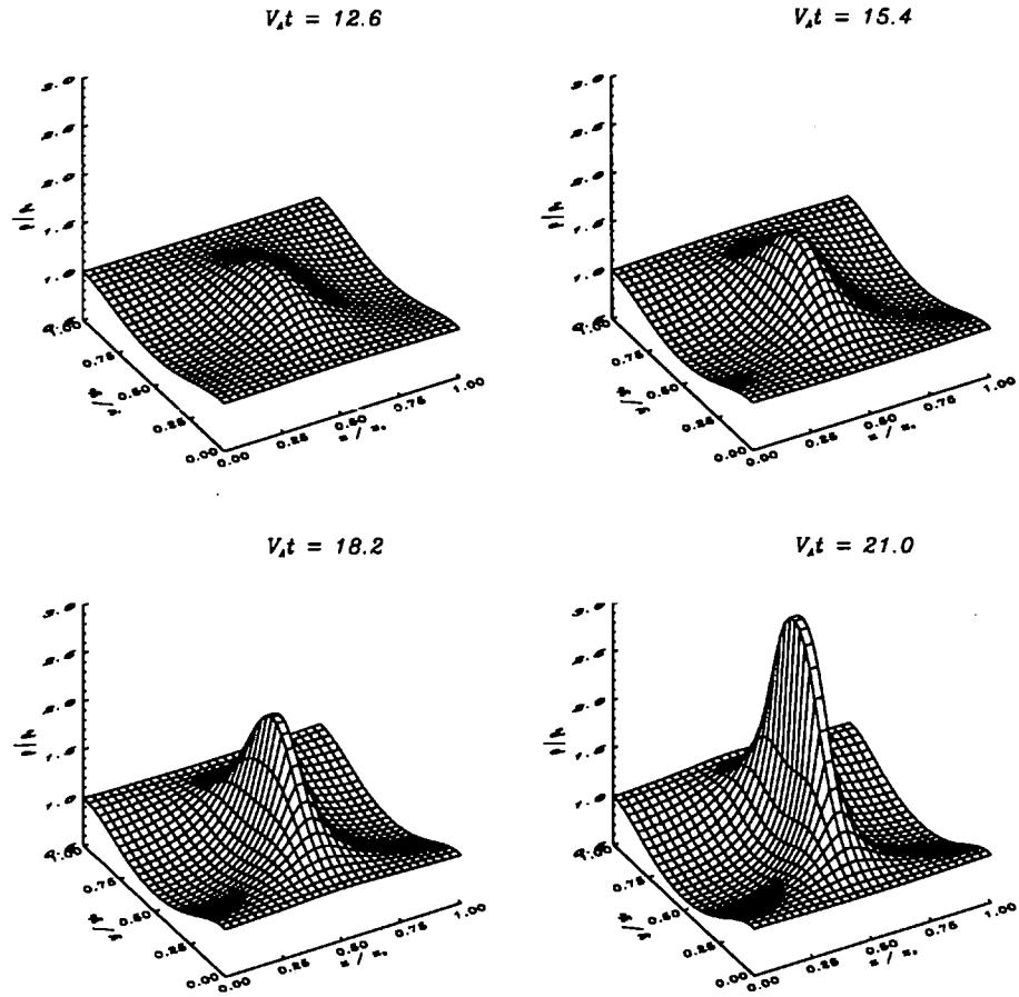
Figure 3.7: Surface plot of the spatial structure of the density at certain times. Initially the fundamental mode with amplitude a = 0.05 is imposed.
