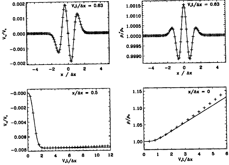
Figure 4.4: A plot of the longitudinal velocity v_x and density \rho . The top panels show the spatial behaviour at an early time V_A t/\Delta x=0.63 . The bottom panels show the early time evolution of the velocity v_x at x/\Delta x=0.5 and the density \rho at x/\Delta x = 0 . The crosses are the full numerical result. The solid line is the quadratically nonlinear solution (4.17). The amplitude parameter a is equal to 0.1.
