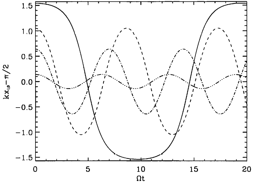
Figure 2.2: Position of bead x_{i,2}(t) for different initial positions kx_{i,0} - \pi/2 (solid line: 1.54, dashed line: 1.05, dot-dashed line: 0.64, triple-dot line: 0.14). The anti-node is at 0. Two nodes are located at \pm\pi/2 .
