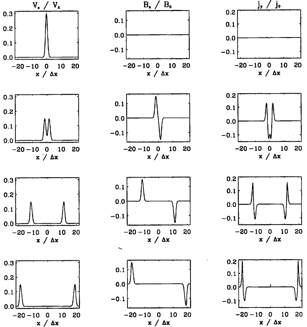
Figure 4.1: A plot of the velocity component v_x , magnetic field component B_x and the current density component j_y as a function of x/\Delta x for four different times (from top to bottom) V_A t/\Delta x = 2 \times 10^{-4} , 1.5, 11.3 and 18.6. The quantity j_0 is defined as j_0 = \Delta x B_0/\mu_0 . The parameter a = 0.15 .
