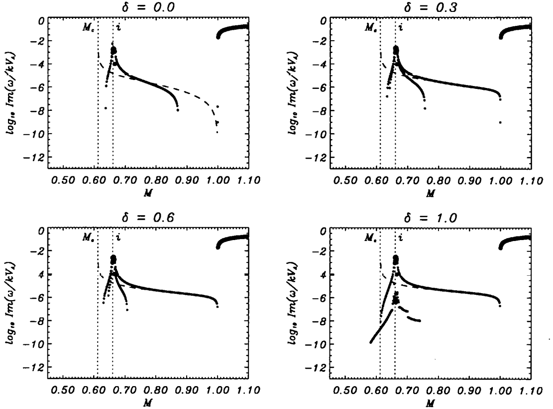
Figure 5.14: Plot of positive values of \text{Im}(\omega/kV_A) as a function of the parameter M on a logarithmic scale, for four values of the parameter \delta , and with \phi = \alpha = \pi/4 , \beta_1 = \beta_2 = 10^{-2} , \eta = 1 , Re = 10^4 and Pr = 10^{-2} . Large dots: K-H instability. Small dots: dissipative instability. Dashed line: leading-order analytical solution (5.78).
