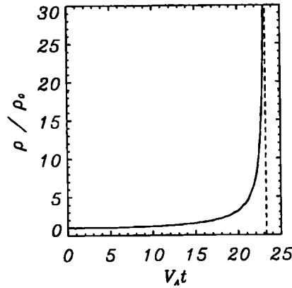
Figure 3.8: Plot of the density at the position of the anti-node in the velocity wave field v_y ( x = 0.5 x_0, y = 0.5 y_0 ) as a function of time. Initially the fundamental mode with an amplitude a=0.05 is imposed.
