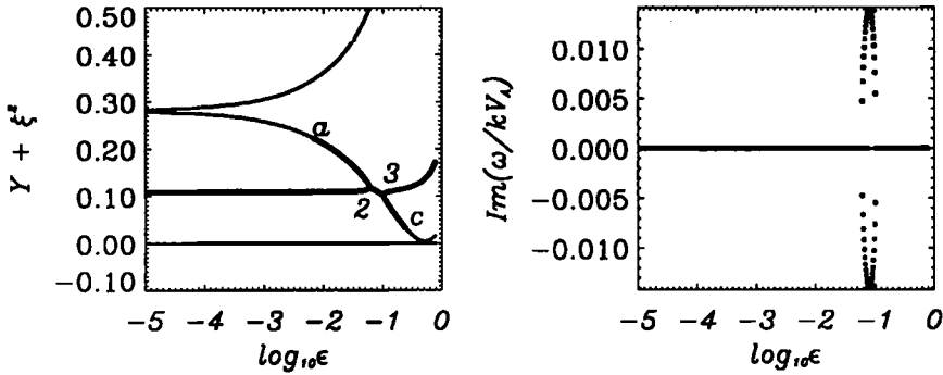
Figure 5.9: Left: Plot of solutions Y + \xi^2 of the dispersion relation (5.54) as a function of \epsilon for M = M_c - 0.14 and \phi = \alpha = \pi/4 . The non-spurious roots are represented by thick lines. The range of the y -axis has been chosen to show the non-spurious roots clearly. Therefore the plot does not show all the roots. The solution branches have been calculated numerically. Right: Plot of \Im(\omega/kV_A) as a function of \epsilon . Non-spurious roots are represented by thick lines.
