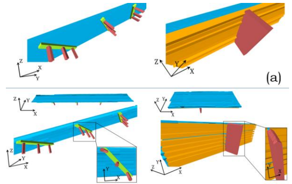
Figure 11: (a) LOD 200 gDTs and (b) LOD 250-300 gDTs. Bridge 1 (L) and Bridge 7 (R)
