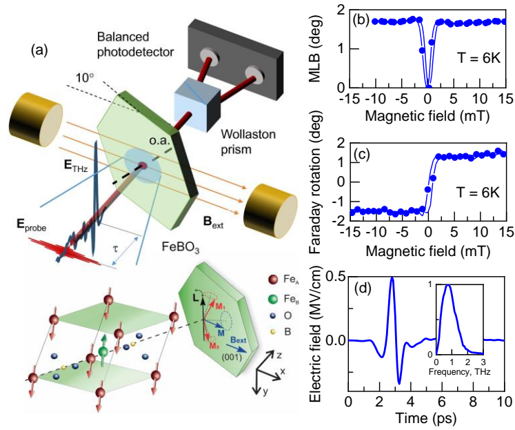
Fig. 1. (a) Schematic of the FeBO 3 crystal structure and experimental geometry. THz and optical pulses are focused onto the FeBO 3 crystal. The diameter of the probe beam is significantly smaller than that of the THz beam. The external magnetic field B_{\text{ext}} is along the x-axis. L and M are antiferromagnetic and magnetization vectors, respectively. \tau is a controllable time delay between the THz pump pulse and the optical probe pulse. o.a. denotes the optical axis (along the z-axis). (b) Ellipticity acquired by linearly polarized light at the wavelength of 800 nm upon propagation along the o.a. as a function of magnetic field applied in the sample plane. (c) Static polarization rotation acquired by linearly polarized light at the wavelength of 800 nm upon propagation through the tilted crystal as a function of magnetic field. The crystal tilt and the orientation of the magnetic field are shown in panel (a). (d) Waveform of the THz electric field and the corresponding Fourier spectrum (inset).
