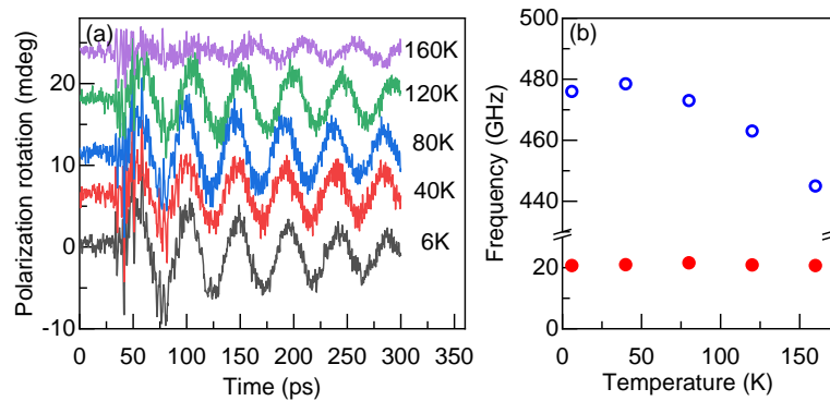
Fig. 4. (a) Optically detected THz induced spin dynamics at different temperatures, indicated near the curves. In the experiment the crystal was tilted around the y -axis over 10°, as shown in Fig. 1a. B_{\text{ext}} = 40 mT. (b) Frequencies of q-AFM (open blue circles) and q-FM (closed red circles) modes of the waveforms from panel (a).
