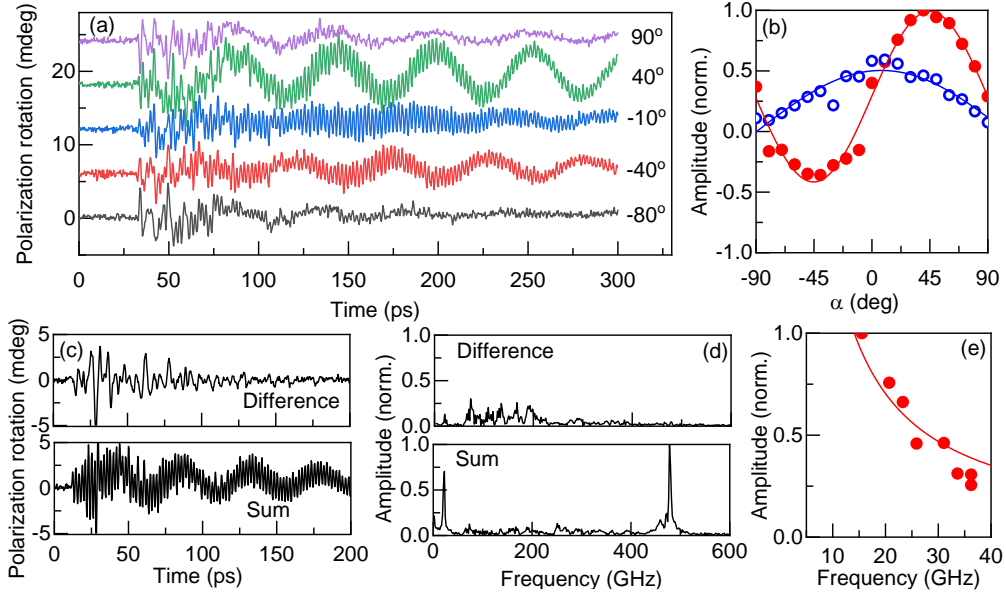
Fig. 3. (a) Optically detected THz induced spin dynamics in FeBO 3 measured for different angles \alpha between the THz electric field and the y -axis. \alpha is shown near each curve. The crystal was tilted around the y -axis over 10°, as shown in Fig. 1a. B_{\text{ext}} = 40 mT, T = 6 K. (b) Normalized Fourier amplitudes of q-AFM (open blue circles) and q-FM (closed red circles) modes from panel (a). Change of sign of the amplitude indicates phase changes. The experimental data are fitted by \sim \cos\alpha (blue curve) and A + B\sin 2\alpha (red curve) (c) Waveforms of the magnetization dynamics after deducing the odd (upper panel) and even (lower panel) parts with respect to the polarity of the applied magnetic field \pm 40 mT. (d) Fourier spectrum of the odd (higher panel) and even (lower panel) waveforms from panel (c). (e) The dependence of the amplitude of q-FM mode on its frequency. Hyperbolic fit is shown by the red curve.
