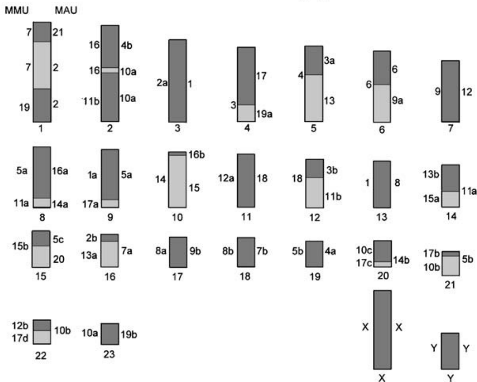
Figure 19 - Ancestral Muroidea karyotype. The homologies of mouse (MMU) chromosomes are shown to the left of the ideogram, and the homologies of golden hamster (MAU) chromosomes are shown to the right of the ideogram.
