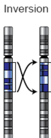
Figure 1 - Chromosomal inversion (image modified from 'Chromosomenmutationen' - Wikimedia commons)
