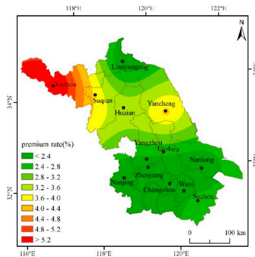
Figure 4. Distribution of actuarially fair premium rate for each city when the deductible amount is 7.5%.
