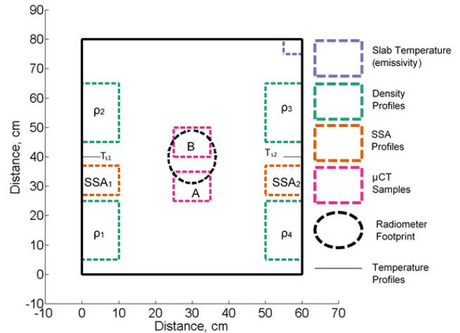
Fig. 1. Approximate locations of the radiometric, macrostructure, and microstructure observations of the ASMEEx snow slabs. Individual \mu CT subsample locations are also shown. Adapted from [31] and [32].
