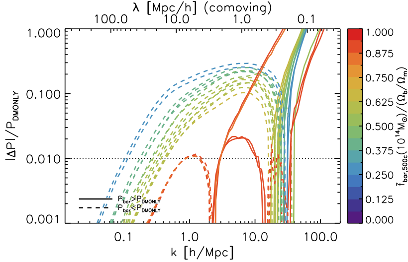
Figure 15. The effect of galaxy formation on cosmo-OWLS and BAHAMAS simulations with 400 h^{-1} \text{ Mpc} boxes. Each simulation is colour coded by its mean baryon fraction within R_{500c} for M_{500c} \approx 10^{14} h^{-1} M_{\odot} haloes, rescaled by the cosmic baryon fraction. The power in the cosmo-OWLS simulations has been renormalized to remove the large-scale offset where applicable (see Section 2.2). The effect of galaxy formation is strongly correlated with the group baryon fraction, a lower fraction corresponding to a stronger suppression of power.
