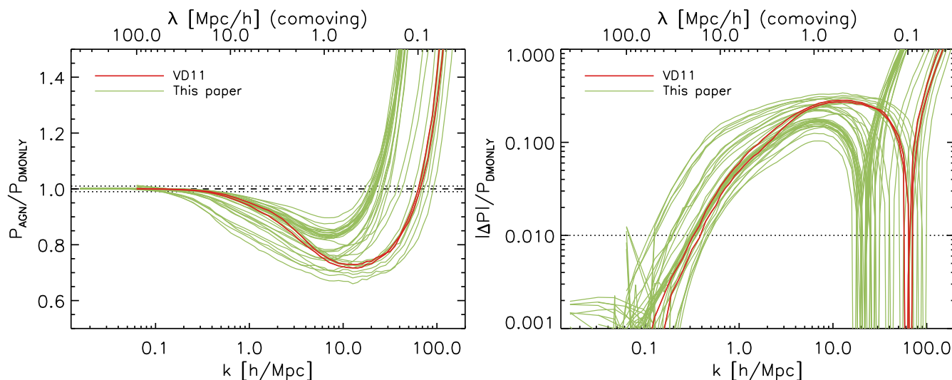
Figure 2. The effect of galaxy formation including AGN feedback on the matter power spectrum. The y-axis shows the change in power relative to a simulation with only dark matter, but otherwise identical initial conditions, linear on the left and logarithmic on the right. Each line shows a simulation with a different feedback strength, cosmology, and/or neutrino mass. The power spectra from the two AGN simulations included in VD11 are highlighted in red (both have identical physics but a slightly different cosmology). The relative effect of galaxy formation is only weakly dependent on cosmology or neutrino mass, and the range in effects seen here is therefore mainly due to changes in the strength of AGN (or stellar) feedback. All subsequent figures will use a logarithmic axis, as we are interested in small changes to the power.
