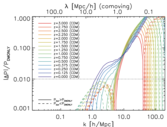
Figure 11. As Fig. 10, but showing the redshift evolution of the back-reaction on the CDM power spectrum. Down to z \approx 1 , the cold dark matter shows increased clustering for k \gtrsim 5 h \text{ Mpc}^{-1} and slightly decreased clustering on larger scales. However, at lower redshifts the dark matter is able to contract on larger scales as well, increasing clustering on all scales k \lesssim 8 h \text{ Mpc}^{-1} .
