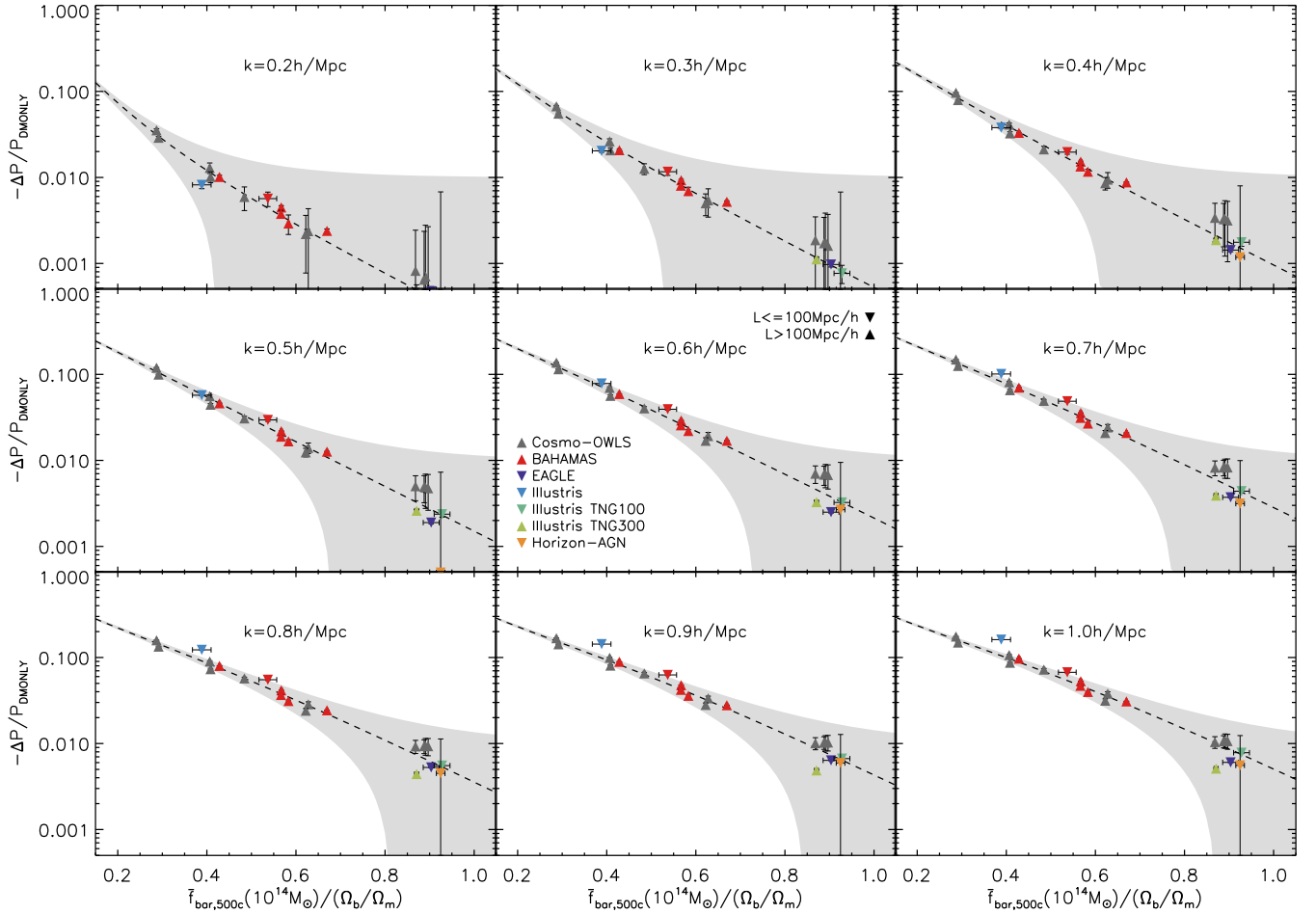
Figure 17. As Fig. 16, but with a logarithmic vertical axis. Each panel shows the relative change in total matter power due to galaxy formation on a different scale, from k = 0.2 h \text{ Mpc}^{-1} in the top left panel through k = 1 h \text{ Mpc}^{-1} in the bottom right panel. The dashed line shows the best-fitting model, fit to the simulations with 400 h^{-1} \text{ Mpc} boxes on all scales k < 1.1 h \text{ Mpc}^{-1} simultaneously (see equation 5 and Table 3), with the grey region showing where the absolute deviation from the fit is \leq 1 per cent.
