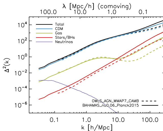
Figure 4. A comparison of the power spectra of the different components for the most realistic simulation included in the VD11 power spectra (dashed lines) and the most realistic simulation in the current set (solid lines, BAHAMAS). The power spectra of OWLS AGN have been renormalized to the Planck 2015 cosmology through the square of the linear growth factor. Despite this, the BAHAMAS simulations generally show stronger clustering in all components except the gas on scales k \lesssim 10 h \text{ Mpc}^{-1} . The primary reason for this is the weaker feedback in BAHAMAS compared to OWLS, allowing more low-mass galaxies to form. On smaller scales, the differences seen here are driven by the change in resolution.
