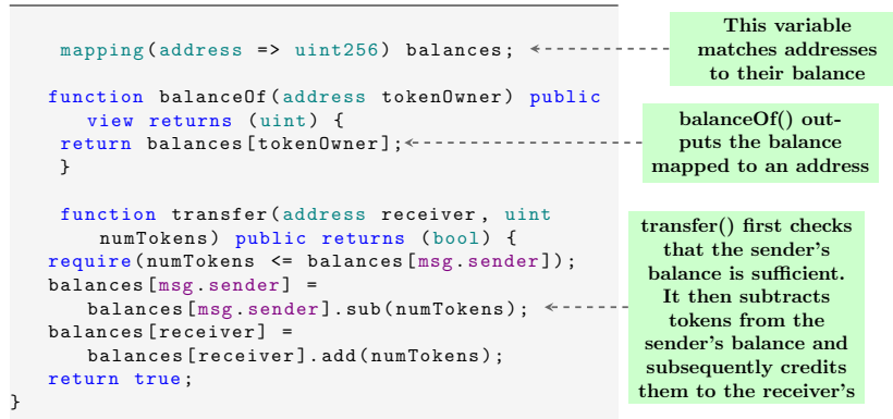
Figure 3: Token Script
