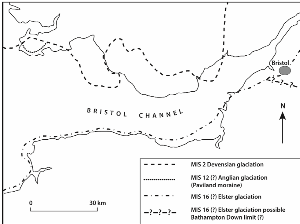
Figure 6. Ice limits in the Bristol region and the Bristol Channel. After Bowen et al. 1986; Campbell et al. 1998; Bowen 2005.
