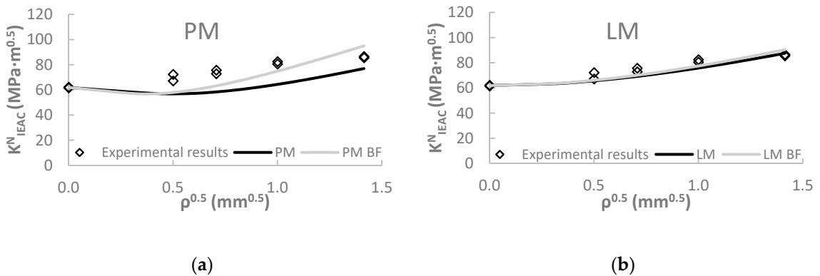
Figure 15. Predictions in S420 steel at 1 mA/cm 2 : (a) PM; (b) LM.
