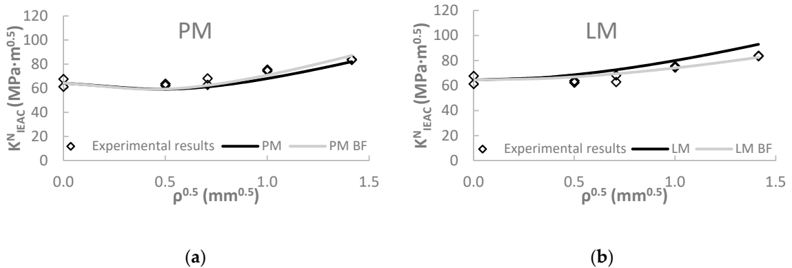
Figure 14. Predictions in S420 steel at 5 mA/cm 2 : (a) PM; (b) LM.
