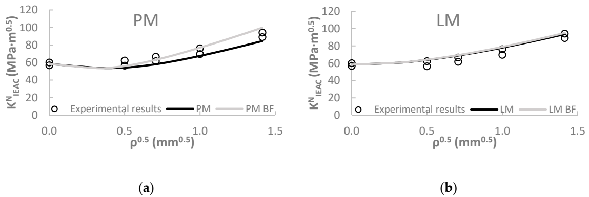
Figure 13. Predictions in X80 steel at 1 mA/cm 2 : (a) PM; (b) LM.
