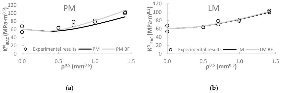
Figure 12. Predictions in X80 steel at 5 mA/cm 2 : (a) PM; (b) line method (LM).
