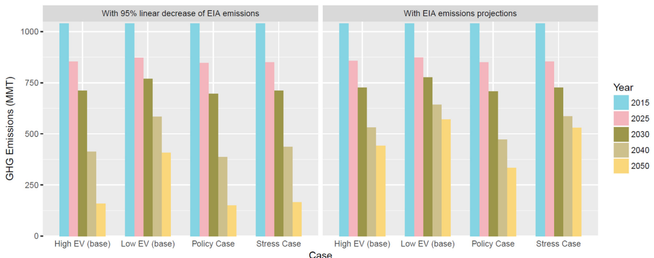
Fig. 8. U.S. LDV greenhouse gas emissions across our scenarios.
