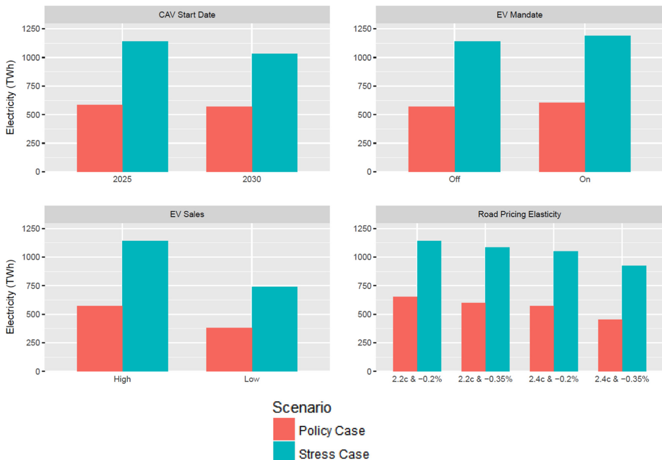
Fig. 7. Sensitivity Calculations (U.S. Electricity for LDVs in TWh).
