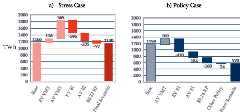
Fig. 6. Components of Estimated Total U.S. Electric Use by LDVs in 2050 (TWh).
