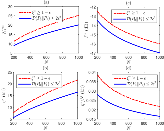
Fig. 3. NP^* , \eta^* , P^* , and \eta/N versus N , where \sigma_b^2 = -5 dB, \sigma_w^2 = 0 dB, \delta = 0.15 , and \epsilon = 0.1 .
