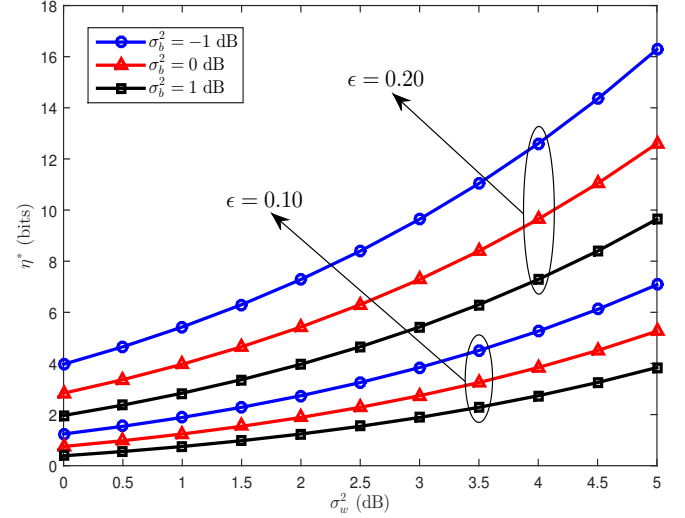
Fig. 4. Maximum \eta versus the noise variance at Willie \sigma_w^2 for different values of \sigma_b^2 and \epsilon , where N = 100 and \delta = 0.20 .
